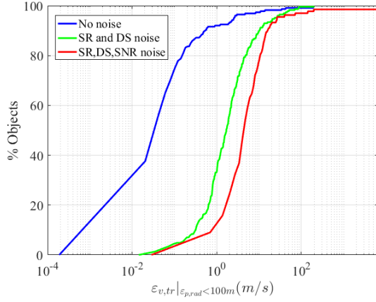
Figure 10. Cumulative error in transversal velocity for all objects with \varepsilon_{p,rad} lower than 100m (unknown object, standard configuration)
