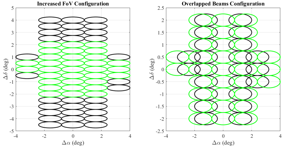
Figure 12. In black: increased FoV configuration (left) and overlapped beam configuration (right). In green: standard beam configuration.
