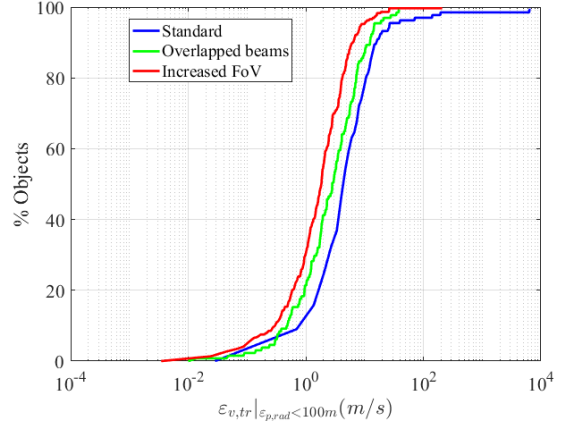
Figure 11. Cumulative error in transversal velocity for objects with \varepsilon_{p,rad} lower than 100m (unknown object, noise in SR, DS, SNR)
