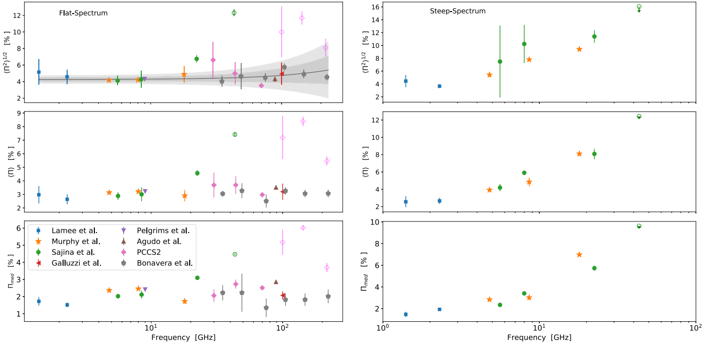
Figure 3. Values of (\Pi^2)^{1/2} (top), \langle \Pi \rangle (center), and \Pi_{\text{med}} (bottom) derived from best-fit lognormal parameters in (4) and (5). Open symbols are data that have not been taken into account for the linear fit in (6). We distinguished FSRQs (left) from the SSRQs (right). In the top left panel, a linear function is fitted from the data to provide a scaling of polarization fraction as a function of frequency. The light and dark shaded area are the 1\sigma and 2\sigma uncertainties, respectively.
