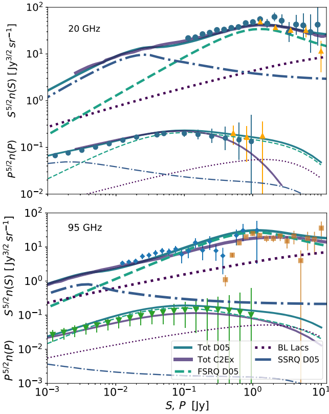
Figure 1. Euclidean differential number counts at (top) 20 and (bottom) 95 GHz. Thick dotted, dashed, dotted-dashed, and solid lines are, respectively, the number counts of BL Lacs, FSRQs, SSRQs, and their total contribution predicted by the D05 model (de Zotti et al. 2005). The thick solid gray line shows the number counts prediction from the C2Ex model (Tucci et al. 2011). Thinner lines follow the same color scheme as the thick ones and refer to polarization number counts, computed via a convolution with a log-normal distribution function fitted from the data. Number count estimates from several surveys are also shown. (Top) The circle data points in the upper curves are data from AT20G (Massardi et al. 2008), whereas upper triangles are from WMAP5-yr survey (K-band, Massardi et al. 2009); in lower curves polarization number counts from a resampling of PACO data (Galluzzi et al. 2018, circles) and from WMAP polarization point source catalog (Lopez-Caniego et al. 2009, upper triangles). (Bottom) Diamonds in upper curves are number counts from SPT (Mocanu et al. 2013), squares are from Planck ERCSC catalog (Planck Collaboration et al. 2011b); the lower triangles have been obtained from a bootstrap resampling of 32 polarized fluxes detected with PACO at 95 GHz.
