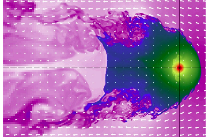
Fig. 16. From Roediger et al. (2015a). Snapshot of a high-resolution simulation of the hot atmosphere of an elliptical galaxy falling into a galaxy cluster. The bottom of the potential well is indicated with the black cross. The arrows show the velocity field of the fluid. Several features can be seen: the cold front at the peak with the KH rolls on the side, the remnant tail in the blue low-velocity area, and the stripped tail trailing behind.
