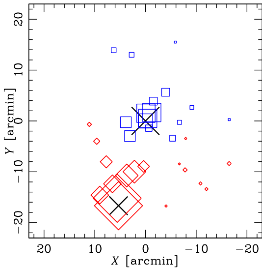
Fig. 13. DS<V> bubble plot for the 33 cluster members. The larger the symbol, the larger the deviation of the local mean velocity from the global mean velocity. Blue squares indicate negative deviations and red rotate squares positive deviations. Crosses indicate the BGC (centre) and LEDA 87445.
