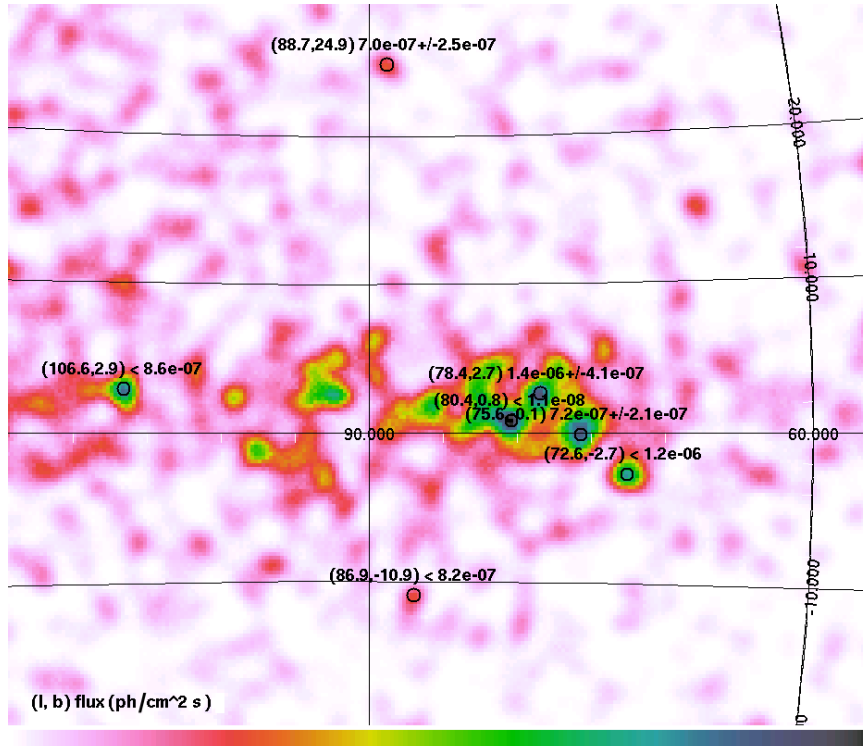
Figure 2.: An example result from the SPOT task. It shows an AGILE gamma-ray sky counts map of the Cygnus region in Galactic Coordinates (l, b) and the estimated flux in photons \text{cm}^{-2} \text{s}^{-1} for each spot confirmed by the ALIKE analysis. Black circles identify the spot position but not the confidence level. The “<” symbol means that the measured flux is an upper limit.
