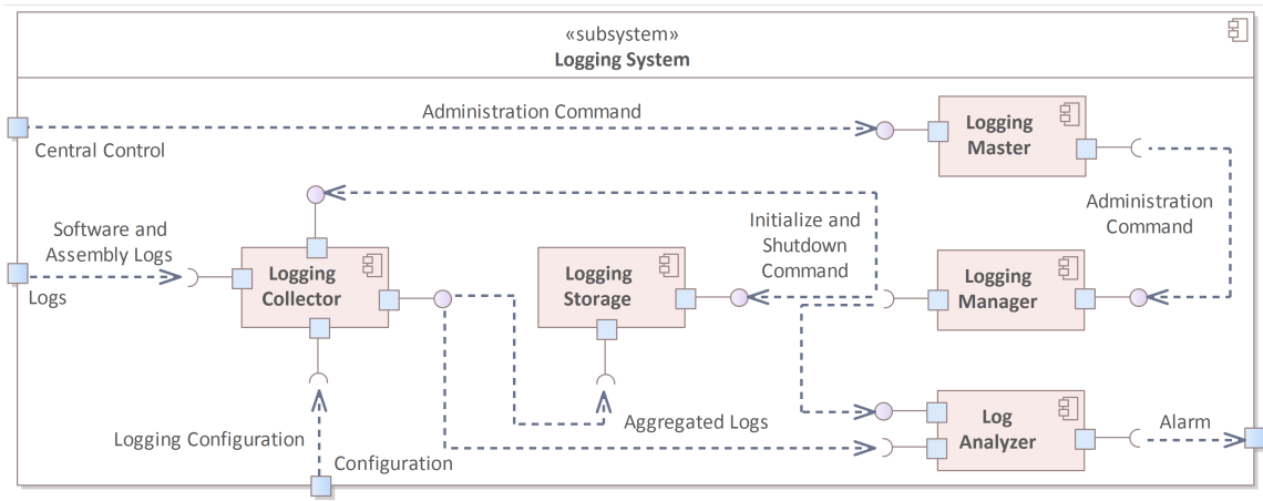
Figure 1: Logical view of LOUD. Log sources are Alma Common Software (ACS) components, OPC UA servers and low-level software.
