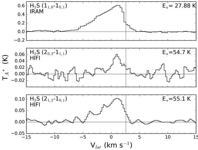
Figure 2. Herschel /HIFI and IRAM-30m/EMIR detections of the H 2 S main isotopologue. The vertical line indicates the cloud velocity V_{\text{sys}} = 2.6 km s -1 .
