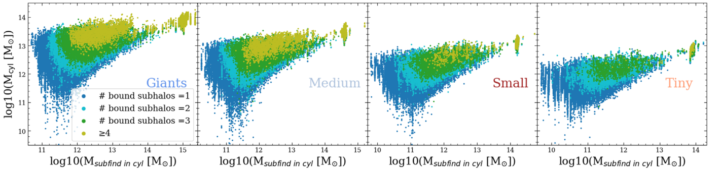
Figure 6. The substructure mass as a function of the most massive bound subhalo within its aperture as given by SUBFIND for the four mass bins (indicated within the plots), with colors denoting the number of bound subhalos within the substructures. The apertures containing a higher number of subhalos are plotted over those with less, to better show their behavior.
