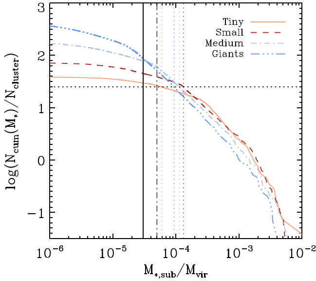
Figure 2. The logarithm with base 10 of the cumulative subhalo abundance per main halo in dependence on the subhalo stellar mass fraction of the main halo. Different colored lines represent the four mass bins. Vertical lines denote two different scalings of M_{*,\text{cut}} . The solid black line scales linearly with the mean virial mass of the galaxy clusters, except for the “tinies” (black dashed–dotted) as they reach the resolution level of at least 100 stellar particles. The colored vertical lines instead scale such as to ensure an approximately constant number of apertures ( \approx 25 , indicated by the horizontal line).
