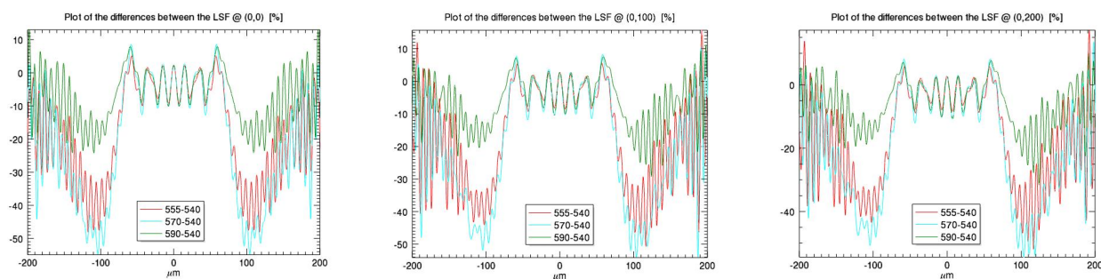
Fig. 6 Differences between the LSF over the wavelengths and the field
