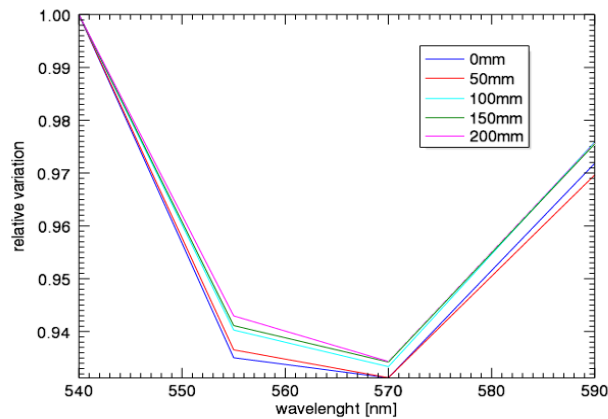
Figure 8: Representation of the variation of the flux with \lambda and field height. Values are normalized to the flux @ Field = [0.0 ; 0.0]
