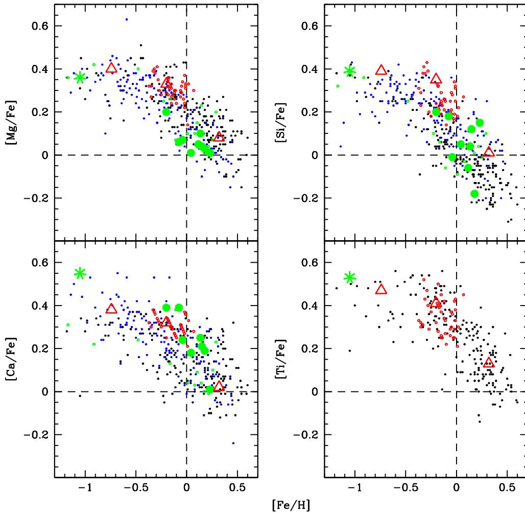
Figure 6. Abundance ratios of [\text{Mg}/\text{Fe}] , [\text{Si}/\text{Fe}] , [\text{Ca}/\text{Fe}] , and [\text{Ti}/\text{Fe}] vs. [\text{Fe}/\text{H}] for GC10812 (big green star) and different samples of bulge and Galactic center giants: Gonzalez et al. (2011) (black dots), Johnson et al. (2014) (blue dots) in the outer bulge from optical spectroscopy, Rich et al. (2007, 2012) (red circles) and Ryde et al. (2016) (green circles) in low-latitude bulge fields, and Ryde & Schultheis (2015) (big green dots) in the Galactic center region from IR spectroscopy. The average abundance ratios of the three stellar populations of Terzan 5 from Origlia et al. (2011, 2013) (big red triangles) are also plotted for comparison. We have rescaled all the abundances to the same solar reference of Grevesse et al. (2007).
