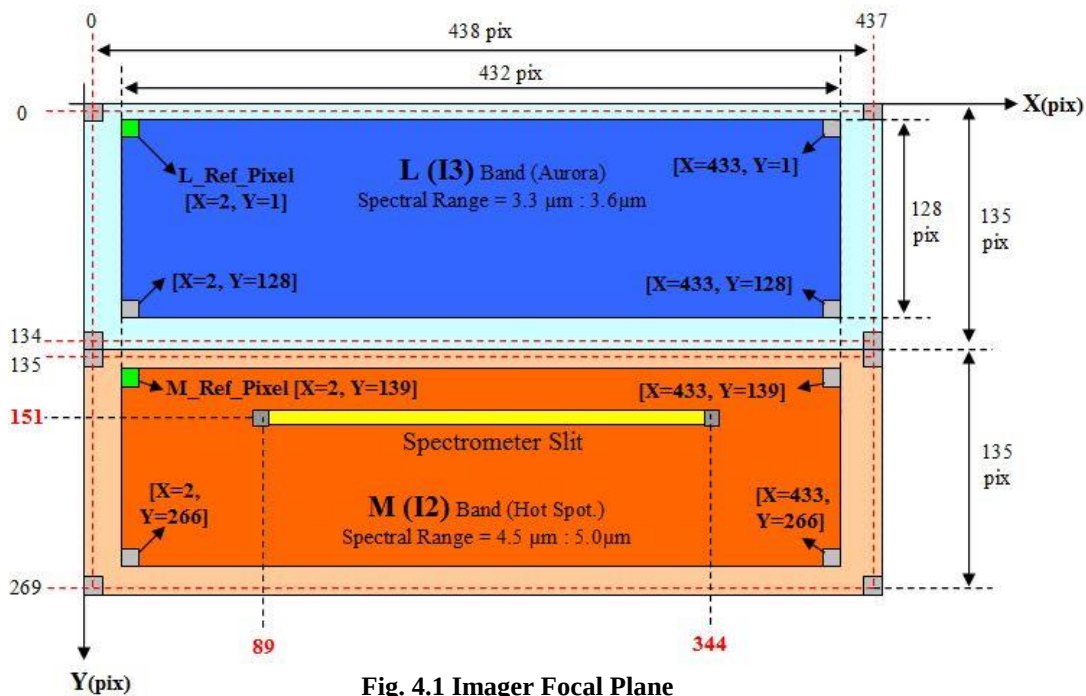
Fig. 4.1 Imager Focal Plane
