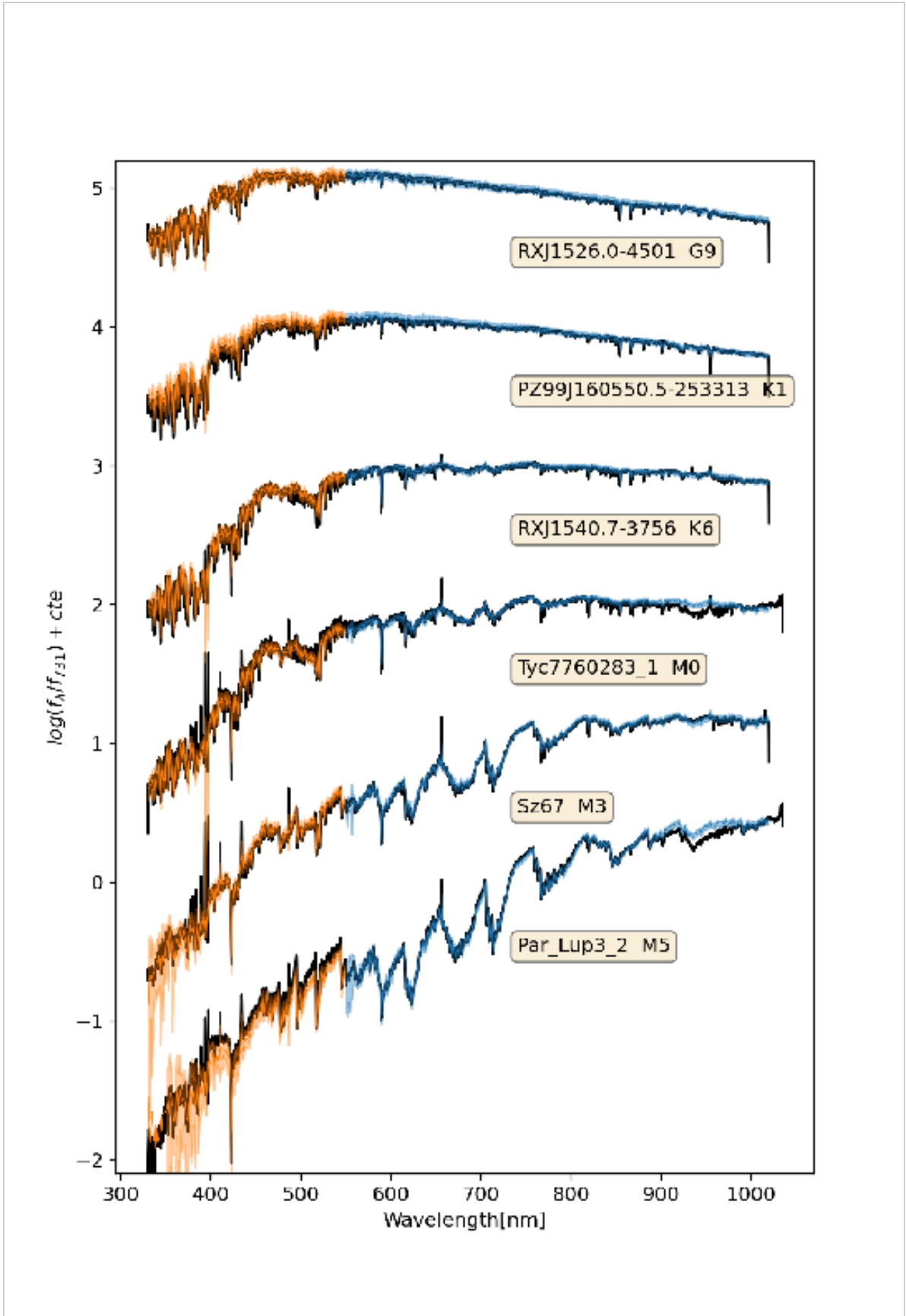
Fig. 7. Comparison between individual Class III templates and the interpolated spectra of the same spectral type. The templates are plotted in black and the interpolated spectra in blue/orange. The transparent blue/orange regions represent the 1-\sigma uncertainties in the interpolated spectra. The blue and orange colours correspond to the wavelength ranges of the X-Shooter VIS and UVB arms respectively. The templates have been convolved with a Gaussian kernel for clarity.
