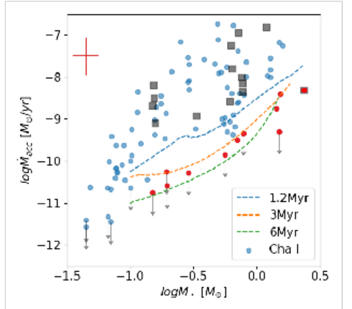
Fig. 13. Mass accretion rate vs. stellar mass for the Chamaeleon I sample presented by Manara et al. (2023) (blue dots) and the Chamaeleon I sample analysed in this work. Objects that have an accretion luminosity lower than the criterion given in equation 6 are marked with a red dot. The limits we derived based on the uncertainties on the chromospheric emission are shown with the blue, orange, and green lines for 1.2, 3, and 6 Myr old objects respectively. The red errorbars indicate the uncertainties on the stellar mass and mass accretion rate. The gray arrows indicate sources listed as upper limits by Manara et al. (2023) .
