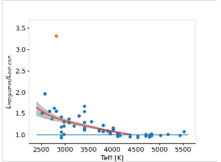
Fig. D.2. Ratio of the luminosities obtained from our spectral integration method and the value computed using the bolometric correction of HHT4. The blue dots indicate the values obtained for the spectra presented here as well as in MTR13 and MFA17. The red line indicates the non-parametric fit, and the shaded area indicates the corresponding 1-sigma uncertainty interval obtained from bootstrapping the non-parametric fitting procedure. The orange point is Par-Lup3-1, which was excluded from this procedure.
