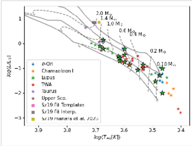
Fig. E.1. HRD containing the different results obtained for Sz19 for comparison the objects analysed here (highlighted with larger black outlined markers) and those analysed by MTR13 and MFA17 are displayed. The model isochrones and evolutionary tracks by Feiden (2016) are also shown. The isochrones are the 1.2, 3, 10 and 30 Myrs ones
