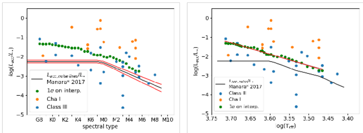
Fig. 12. SpT and T_{\text{eff}} dependency of the accretion noise \log(L_{\text{acc,noise}}/L_*) values obtained from interpreting the uncertainties in the Balmer and Paschen continuum ( < 500 nm) on our model Class III spectra as accretion (Green dots). The blue dots illustrate the \log(L_{\text{acc,noise}}/L_*) values obtained when fitting the Class III spectra with an accretion slab model. The results obtained for the PENELLOPE Chamaeleon I sample is indicated with orange dots. The black line shows the L_{\text{acc,noise}} relationship measured from the emission lines by MFA17 and the red lines on the left show the uncertainty thereon. On the right, the red line illustrates the best fit to the \log(L_{\text{acc,noise}}/L_*) values.
