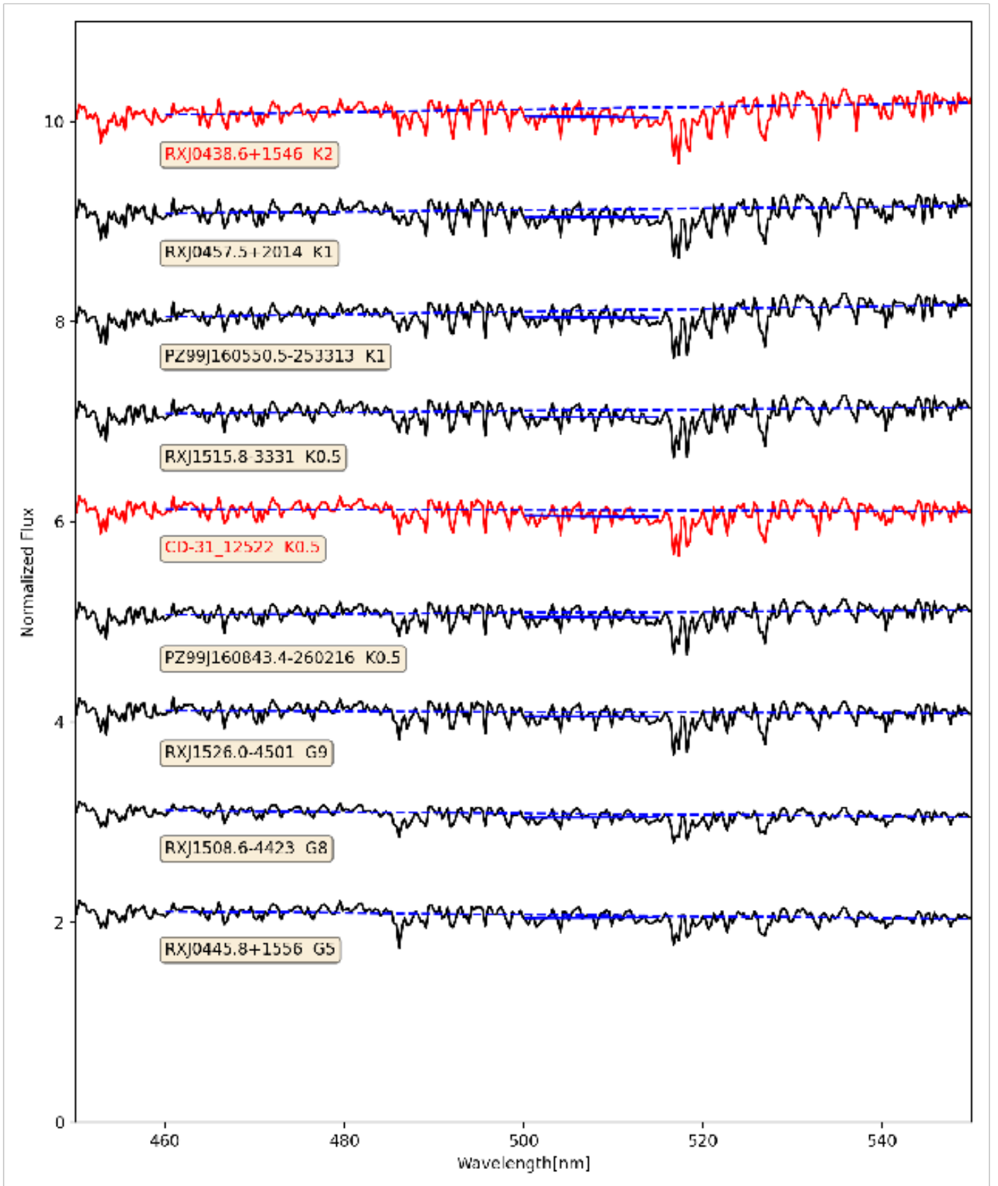
Fig. G.7. X-Shooter spectra of Class III YSO with spectral types ranging from K2 to G5 ordered according to SpT and normalized at 520 nm. (continued on Fig. G.7). Spectra presented in this work are indicated in red and spectra from the samples of MTR13 and MFA17 are indicated in black.
