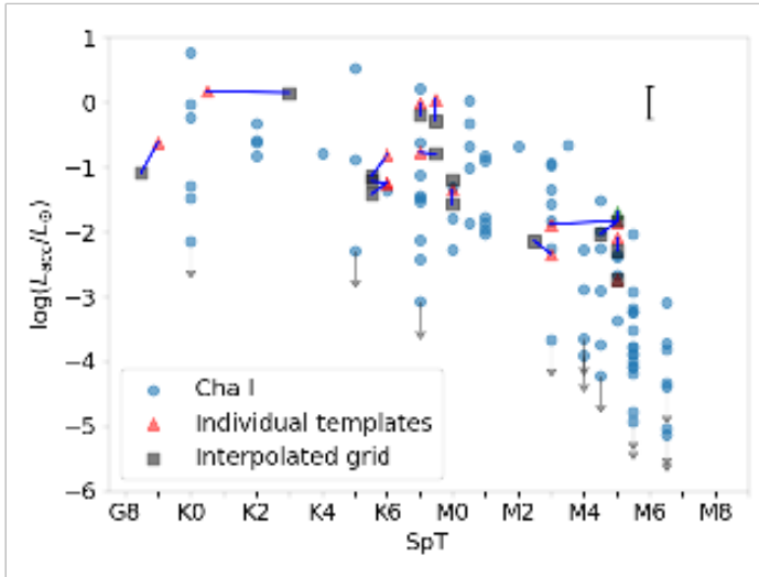
Fig. 9. Accretion luminosities vs. spectral type as obtained using FRAPPE (gray squares) and obtained using the method of Manara et al. (2013b) (red triangles). Results obtained for the same target with the two methods are connected with a blue line. The green triangle indicates the M5 solution of WZ Cha. The light blue circles are the nearly complete Chamaeleon I sample presented by Manara et al. (2013a). The black errorbars indicate the uncertainties on the accretion luminosity. The gray arrows indicate sources listed as upper limits by Manara et al. (2023).
