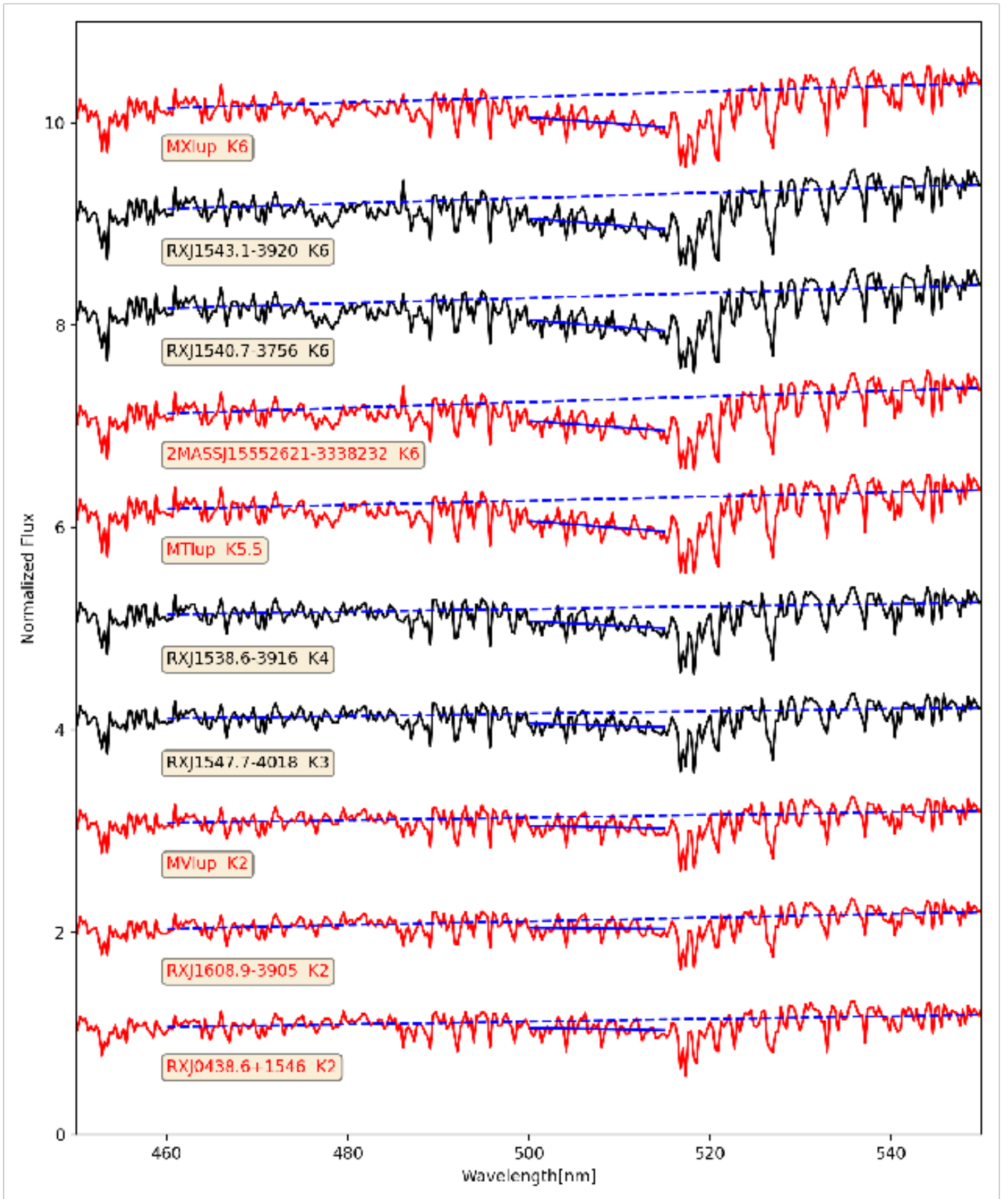
Fig. G.6. X-Shooter spectra of Class III YSO with spectral types ranging from K6 to K2 ordered according to SpT and normalized at 520 nm. (continued on Fig. G.7). Spectra presented in this work are indicated in red and spectra from the samples of MTR13 and MFA17 are indicated in black.
