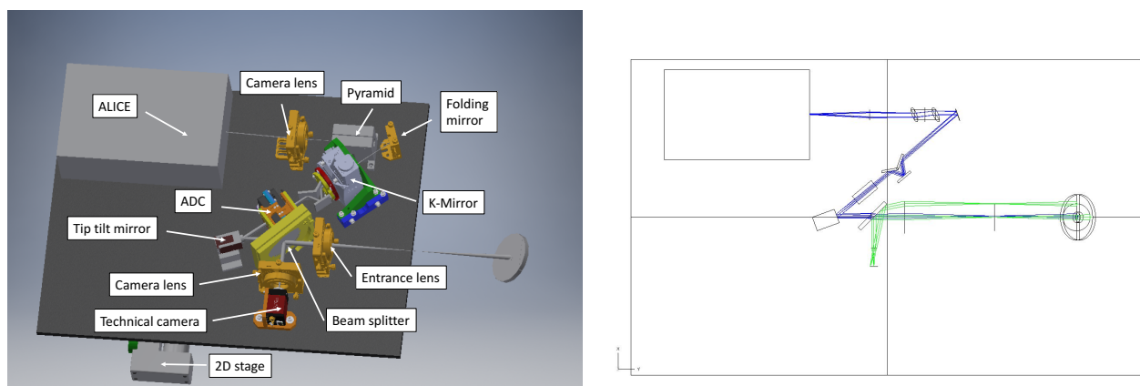
Figure 2: (left) SCAO module components overview and (right) Optical layout of the SCAO WFS. Green color highlights the TV channel light path while blue color the WFS channel.
