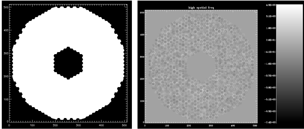
Figure 3 Pupil of the E-ELT (left) and High spatial frequency error sample(right).
