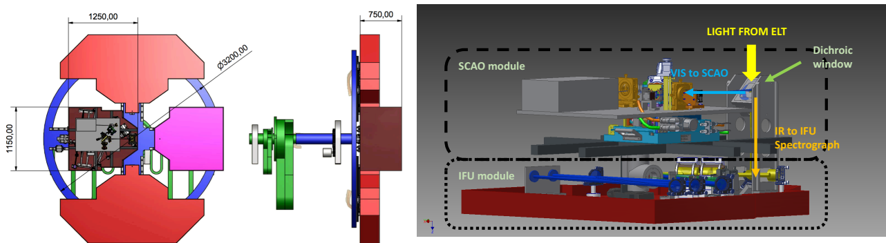
Figure 1 (left) The IFU-SCAO module is located into the Nasmyth rotator structure. (right) Mechanical 3D view of the module
