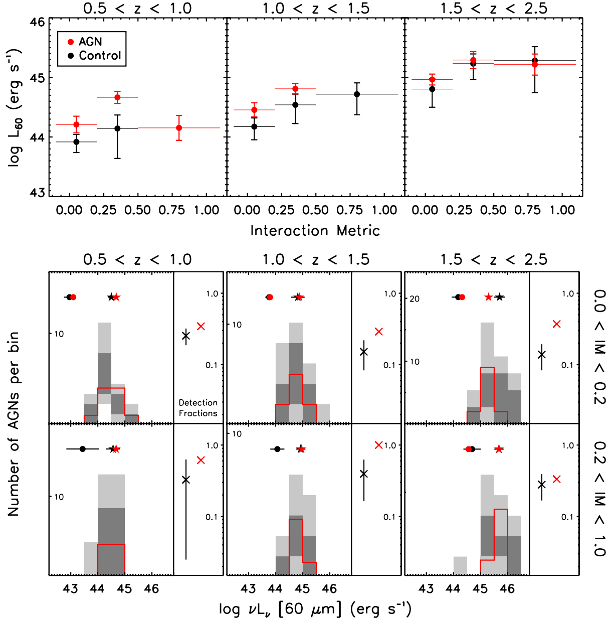
Fig. 14. Mean 60\ \mu\text{m} monochromatic luminosities ( L_{60} ) and luminosity distributions of AGNs and inactive control galaxies in GOODS-S, as a function of visual Interaction Metric (IM). Panels left to right span three distinct bins in redshift. In the top row , the mean L_{60} from combinations of detections and stacks are compared in bins of IM. In the lower two rows , each panel is split into two subpanels . L_{60} distributions and PACS detection fractions for AGNs and inactive galaxies are plotted in the left subpanels for two coarse bins in IM. PACS detection fractions are shown in the right subpanels . Details of the plot are identical to those of Fig. 13, except for a difference in the structural measure. See Sect. 4.2 for a discussion.
