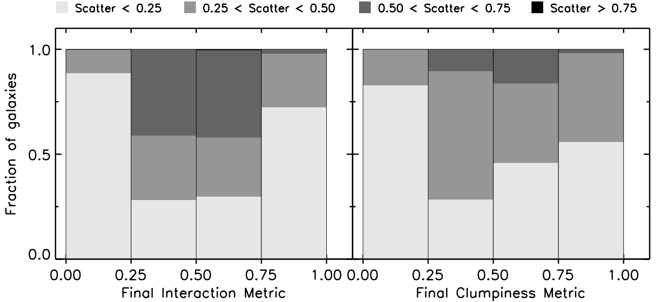
Fig. 1. The breakup of the mean scatter of visual classification metrics for galaxies at 0.5 < z < 2.5 binned by their final mean metric value. The mean scatter for a galaxy is defined as the average absolute value of the difference of the metric between pairs of classifiers for that galaxy. Galaxies with larger scatter have a larger level of disagreement between the individual visual classifications. The relative number of galaxies in four ranges of scatter are shown, represented by lighter to darker grayscale towards increasing scatter. Galaxies are binned by the final interaction metric (IM, left panel ) and the final clumpiness metric (CM, right panel ).
