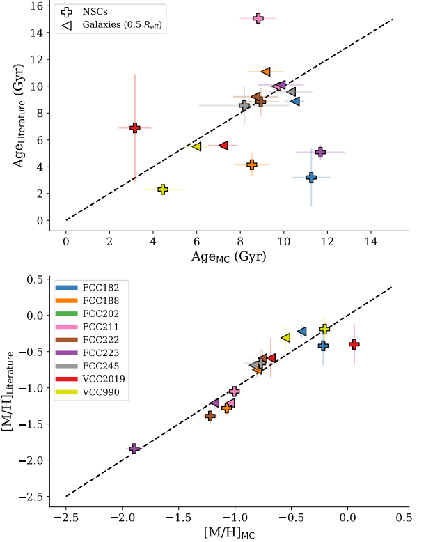
Fig. 7. Comparison of ages ( top ) and metallicities ( bottom ) of the NSC (crosses) and host galaxy (triangles, at 0.5 R_{\text{eff}} ) from the literature and this work. The different colours refer to the different galaxies. VCC 990 was analysed by Paudel et al. (2011), VCC 2019 by Spengler et al. (2017), and the other galaxies by Johnston et al. (2020). The dashed lines refer to the one-to-one relation.
