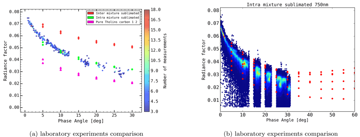
Figure 15. (a) Comparison phase curves of dry laboratory samples and NAC F88 fly-by area for phase angle smaller than 35^\circ at 750 nm. For both data, it was selected measurements at incidence angle equal to zero. The dry samples are the sublimated intramixtures and intermixtures, and an assemblage of tholins (33 per cent)+carbon black(66 per cent). (b) Best match: sublimated intramixture. The scatter of measurements well represent the disc behaviour observed in the fly-by phase curve. The lack points at \alpha < 5^\circ do not allow us to infer any information about the opposition surge.
