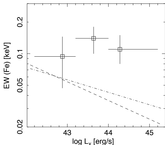
Fig. 16: Plot of narrow Fe K line EW against X-ray luminosity obtained from the three luminosity slices of unobscured AGN (Table 9). The dashed and dash-dotted lines indicate the I-T effect obtained for nearby AGN by Bianchi et al. (2007) and Shu et al. (2012), respectively.
