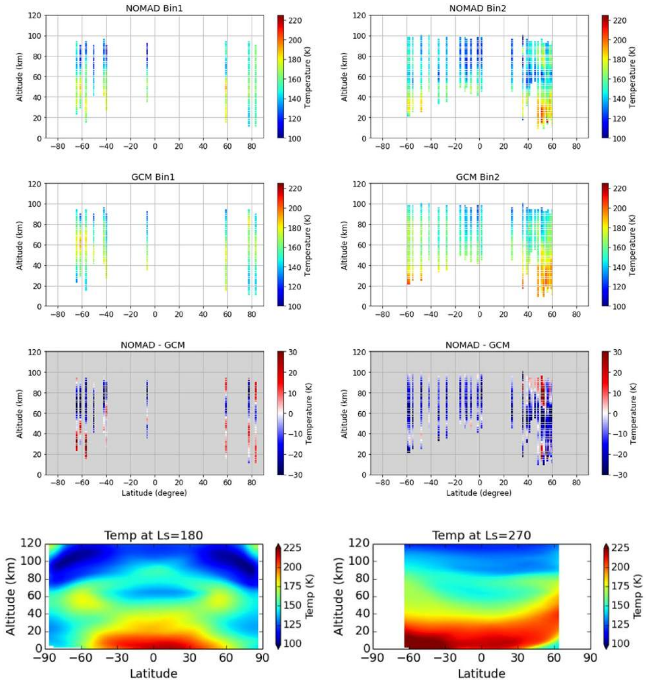
Figure 12. Latitudinal distribution of the retrieved Nadir and Occultation for Mars Discovery (NOMAD) temperatures in two seasonal periods. Left panels: period L_s = 160^\circ – 190^\circ ; right-hand side: period L_s = 285^\circ – 305^\circ . Top panels: NOMAD retrieved temperatures; second from top: global climate models (GCM) temperatures at the same locations and local times; third panels from top: difference NOMAD-GCM; and bottom panels: altitude/latitude cross sections of the Laboratoire de Météorologie Dynamique temperatures at L_s 180^\circ and 270^\circ , for comparison.
