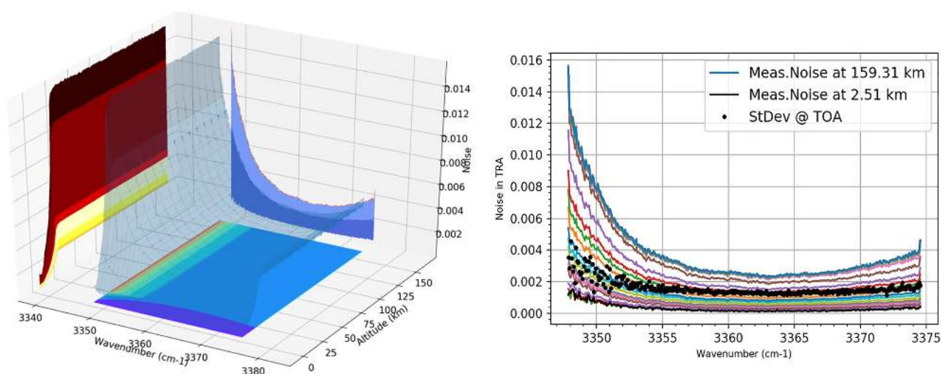
Figure 4. Measurement noise in transmittance in the order 149 of scan 20180423_204351_1p0a_SO_A_I, typical of all scans in this diffraction order. Left panel, variations in the spectral and altitude dimensions. Right-hand panel: alternative view of the projection onto the wavenumber-noise plane to appreciate better the quasi-random variations; each line represents a noise spectrum (at one tangent altitude). The black-dots are the standard deviation of transmittance vertical profiles near the top of the atmosphere. The color scales in both panels are arbitrary. See text for details.
