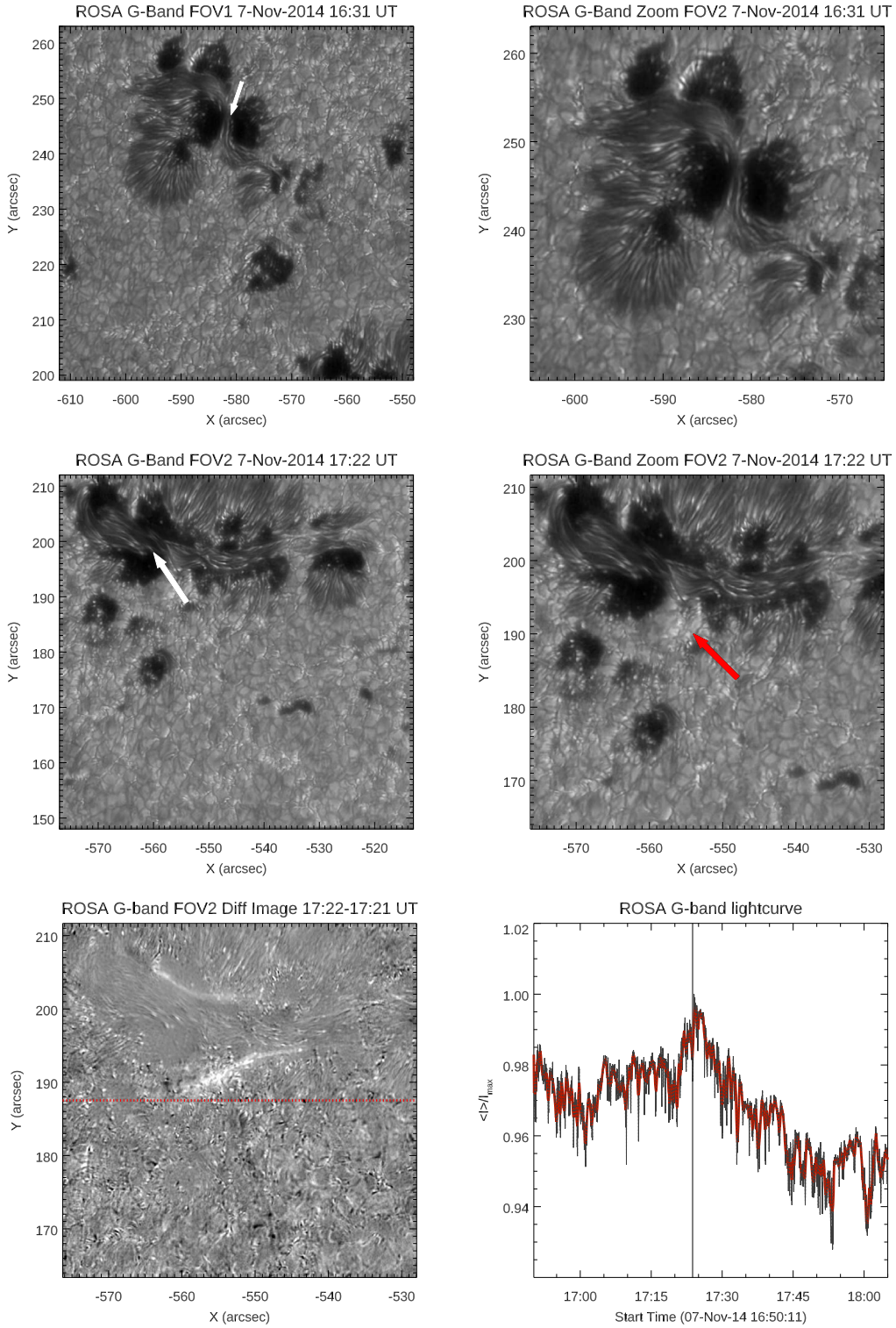
Figure 3. ROSA G -band images of AR 12205. Top panels: (left) the entire FOV1, at 16:31 UT. The white arrow indicates the \delta -spot A. (Right) Zoomed image from ROSA FOV1 showing the details of \delta -spot A, characterized by the presence of sheared penumbral filaments within the two opposite magnetic polarities. Middle panels: (left) the entire FOV2 at 17:22 UT, during the rise phase of the X1.6 flare, a few minutes before the peak. The white arrow indicates the \delta -spot B. (Right) Zoomed image from ROSA FOV2 showing the location of a ribbon observed in the continuum (red arrow) at 17:22 UT. Bottom panels: (left) difference imaging of zoomed FOV2, showing the ribbons at a time close to the peak of the X1.6 flare. The red dotted line separates the zoomed FOV2 into two halves. (Right) G -band lightcurve relevant to the upper half of the zoomed FOV2, where the ribbons are observed. The red line represents a smoothed trend. The vertical line indicates the X1.6 flare peak. An animation of the G -band images relative to the zoomed FOV2 is available. The video begins at 16:50:11 UT and ends at 17:40:03 UT. The real-time duration is 43 s. Note the passage of the ribbon at around 17:22 UT.
