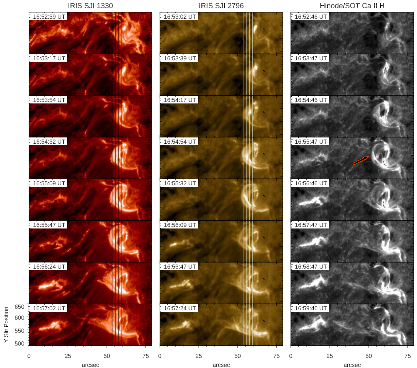
Figure 6. The evolution of the flaring site around the northern \delta -spot A at the beginning of the X1.6 flare, on 2014 November 7, in three different wavelengths: IRIS SJI 1330 Å (left), IRIS SJI 2796 Å (middle), and Hinode /SOT Ca II H (right). In the IRIS SJIs, the dashed vertical lines indicate the raster positions during the acquisition time. The arrow in the Ca II H filtergram indicates the expanding flux rope, which is launched during the sequence.
