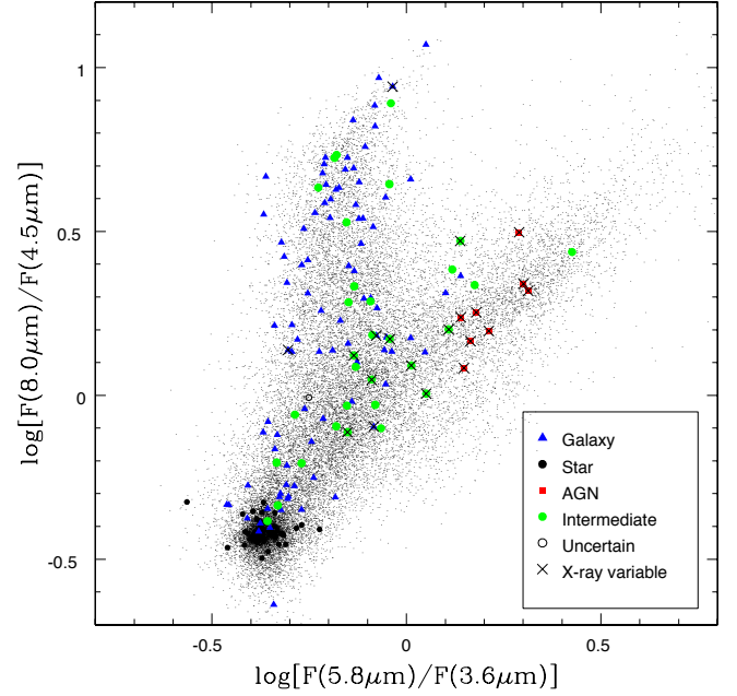
Fig. 12. The 8.0/4.5\text{ }\mu\text{m} flux ratio versus the 5.8/3.6\text{ }\mu\text{m} flux ratio. The small black dots refer to the SWIRE sample analysed by Vaccari et al. (2010, and in prep.). The largest symbols represent the XMMOMCDFS sources with available IR data from the previous sample, with the same meaning as the symbols in Fig. 3. In addition, the crosses indicate X-ray variable sources according to Paolillo et al. (2004, and in prep.). Symbols are also reported in the legend.
