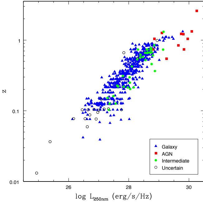
Fig. 9. L_{250 \text{ nm}}\text{-}z plane for the extragalactic objects. Symbols and colours are defined as in Fig. 3 and reported in the legend.
