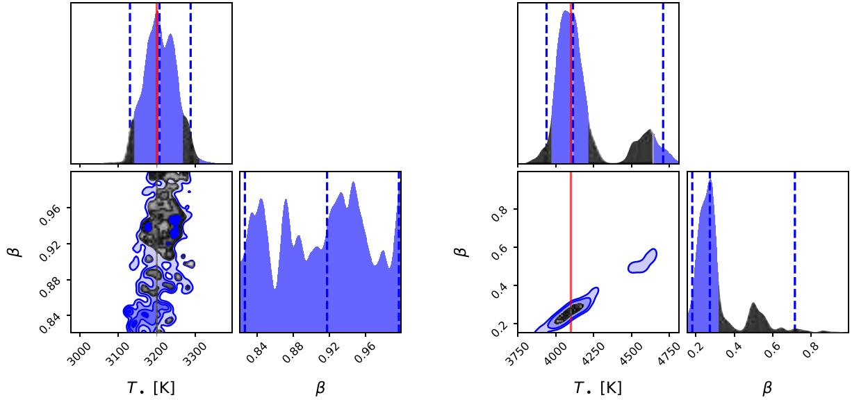
Figure 8. Left: T_s and \beta posterior distributions for the 14.5 K mag, M star observed with NIRSpect/Prism and a T_s = 3200 K occulted starspot, with \theta = 0^\circ . While the occultation signal is strong enough to exclude T_s = T_\star , the high \beta_{\min} forces the solution towards a warm spot (see Section 4.3). Right: T_s and \beta posterior distributions for the 7.5 K mag, K star observed with NIRCcam/F150W2 + F322W2 and a T_s = 4100 K occulted starspot, with \theta = 0^\circ (see Section 4.4). The 95 per cent credible intervals are represented with blue vertical dashed lines, while the true T_s value is indicated with a red vertical line.
