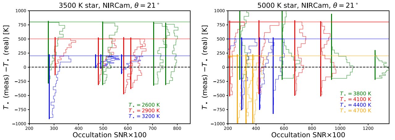
Figure B3. Same as Fig. B1 for spots at 21° stellar latitude, for the M (left) and K (right) scenarios observed by NIRCcam/F150W2 + F322W2.
