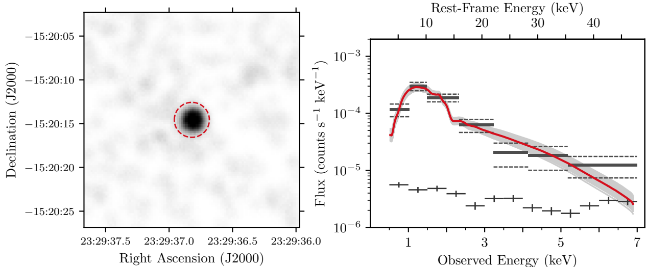
Figure 1. Left: 0.5–7.0 keV Chandra observation of PJ352–15, smoothed by a Gaussian kernel of width 0''.75 . The 2''.0 radius extraction region used for photometry and spectroscopy is indicated by the red circle. Right: X-ray spectrum of PJ352–15. Data (dark gray) are binned for ease of display, but were not binned during fitting. The best-fitting spectrum is shown in red, while 100 spectra with \Delta C \leq 2.30 from our Monte Carlo analysis are shown in gray. The background spectrum is shown in dark gray error bars at the bottom.
