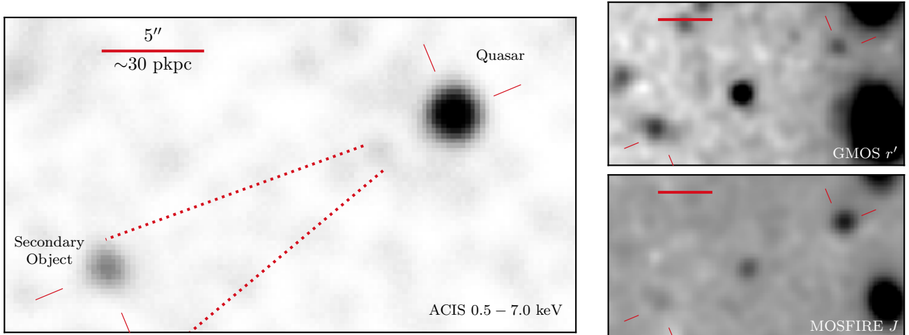
Figure 5. Multiwavelength observations of the area around PJ352–15, showing the broad X-rays (left), r' (top right), and J (bottom right). All images show the same field of view, with north pointing up and east to the left, and a 5'' scale bar is shown for reference. An object (bottom left of all panels) is seen in X-rays \sim 100 kpc from the quasar (top right of all panels) at the counter angle of the jets (position angles of 110^\circ and 130^\circ are indicated by the dotted lines, for reference); both objects are indicated in all images by red reticles. This source is also seen in the observed optical and NIR imaging, as discussed in the text. Additional sources present in the r' and J images have no X-ray counterparts.
