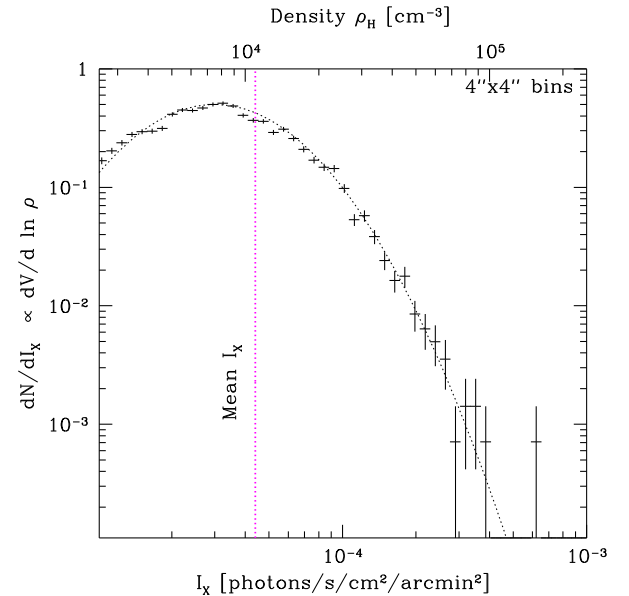
Figure 5. Observed Probability Distribution Function of the X-ray surface brightness I_X in the reflected component for 4 arcsec bins, corresponding to \sim 0.16 \text{ pc} . In the optically thin limit \text{PDF}(I_X) is essentially \text{PDF}(\rho) with proper transformation of arguments. The upper horizontal axis shows the density obtained by converting I_X to the gas density, using equation (5) in the limit of an optically thin cloud. The decline at large densities is either due to averaging over the bin’s volume, opacity effects or the paucity of small and dense clumps. The \text{PDF}(I_X) based on the existing data is strongly affected by the photon counting noise, especially at low flux levels.
