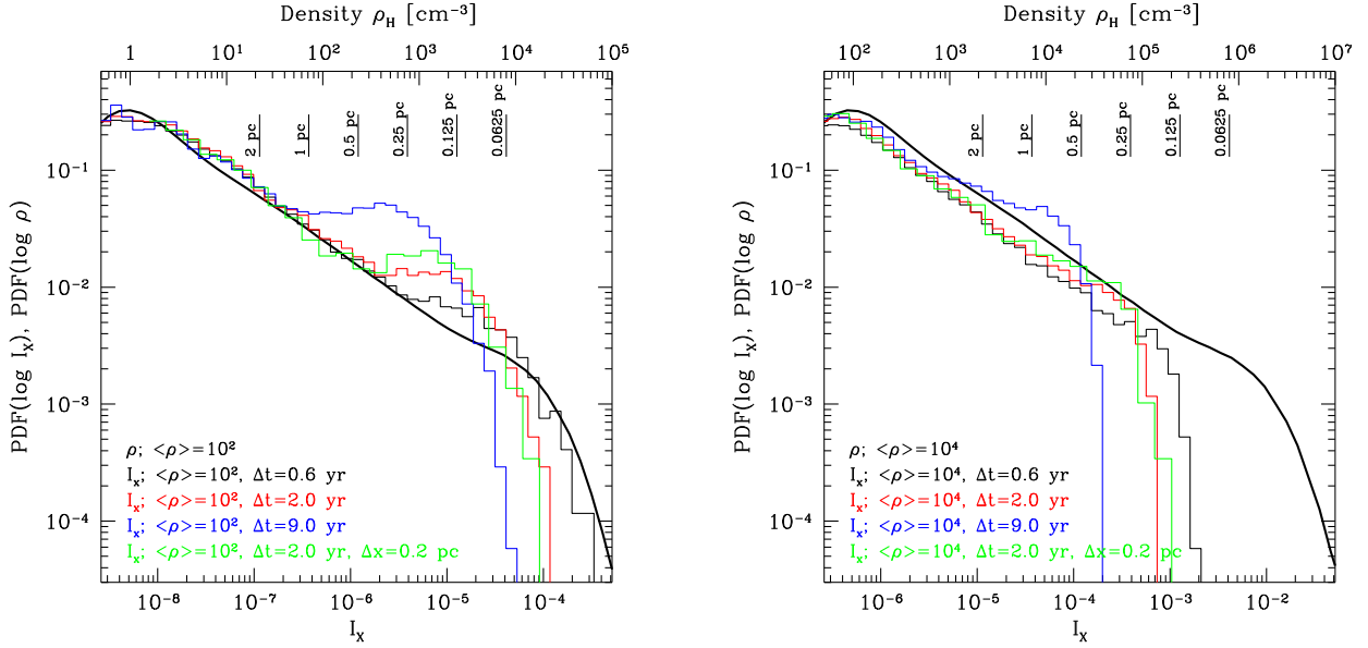
Figure 4. Simulated \text{PDF}(\rho) and \text{PDF}(I_X) for a molecular cloud illuminated by an X-ray flare from Sgr A*. The left- and right-hand panels correspond to the clouds with mean hydrogen densities 10^2 and 10^4 \text{ cm}^{-3} , respectively. In both plots the thick black line shows the \text{PDF}(\rho) ( \rho is shown in the upper horizontal axis), while the histograms correspond to the observed \text{PDF}(I_X) for flares with different durations ( I_X is shown in the lower horizontal axis). The two horizontal axes are aligned such that in the optically thin limit a given value of \rho corresponds to the value of I_X , so that \text{PDF}(\rho) and \text{PDF}(I_X) can be compared directly. The cloud in the left-hand panel is optically thin and for a short flare ( \Delta t = 0.6 \text{ yr} the black ‘observed’ histogram reproduces well \text{PDF}(\rho) ). As the duration of the flare increases, the size of the illuminated region along the line of sight \Delta z becomes larger than the size of small and dense cores and the value I_X moves to the left, forming a distinct bump in the \text{PDF}(I_X) (see the text for details). For the denser cloud (right-hand panel), small clumps become optically thick and a cut-off in \text{PDF}(I_X) develops towards high-density end. These simulations show that it is possible to recover \text{PDF}(\rho) for the low-density part of the distribution, provided that the duration of the flare is sufficiently small.
