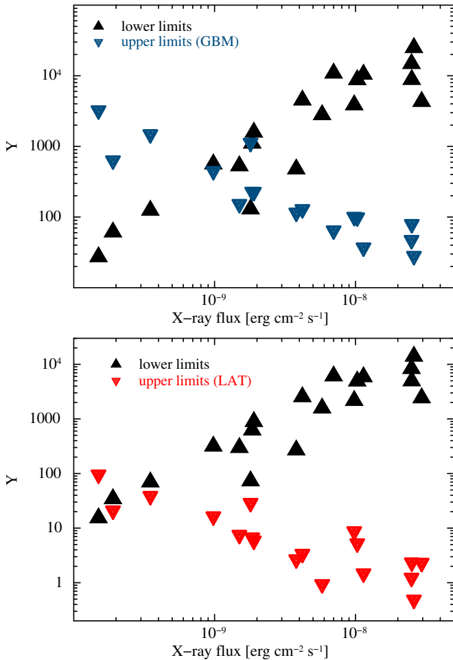
Figure 2. Top panel: constraints on the Y -parameter as a function of the observed X-ray flux. The lower limits on the Y -parameter were calculated according to Equation (25) for an IC peak frequency \nu_\gamma = 10 MeV. Upper limits were derived from Fermi /GBM observations. Bottom panel: constraints to the Y -parameter as a function of the observed X-ray flux. The lower limits on the Y -parameter were calculated according to Equation (25) for an IC peak frequency \nu_\gamma = 100 MeV. Upper limits were derived from Fermi /LAT observations.
