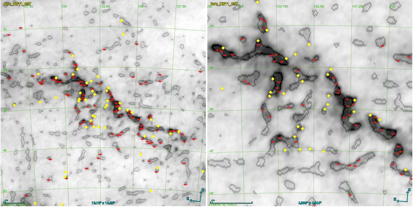
Fig. 1. Left: A 10^\circ \times 10^\circ mid-Galactic-latitude ( b^\text{II} \approx 45^\circ ) region of the Planck 857-GHz map superimposed on the PCCS2+2E filament mask (grey contours). PCCS2 sources are yellow diamonds and PCCS2E sources are red triangles. The selected region contains complex backgrounds with localized features such as filaments and cirrus, causing the mask to break up into numerous islands. Many PCCS2+2E sources trace these structures, suggesting that some of the sources are parts of filamentary structures broken up by the source-finder and not genuine compact sources. Right: The central 4.9^\circ \times 4.9^\circ of the picture on the left, showing more clearly the spatial distribution of the PCCS2 and PCCS2E sources relative to the mask.
