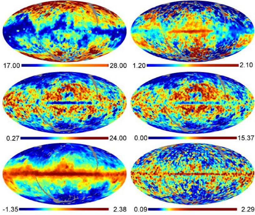
Fig. 19. Top: MBB parameters fitted to the background, with T(K) on the left and \beta on the right. The high-temperature region at ( l = 155^\circ; b = 77^\circ ) is artificially created by strong artefacts in the IRIS data. Middle: Inverse relative uncertainty T/\Delta T (left) and \beta/\Delta\beta (right) of the MBB parameters. Bottom left: Reference background brightness, \log(\text{Jy pixel}^{-1}) , evaluated at 857 GHz. This is the value at 857 GHz of a multifrequency fit, not the value directly measured at 857 GHz. Bottom right: \log(\text{RELTH}) , computed with \alpha = 5\% (see Eq. 9). On all panels there is a region at ( l = 208^\circ; b = -18^\circ ) of extreme values and uncertainties caused by artefacts present in the IRIS data. The colour bars have been histogram-equalized. regions are either inside the IRIS mask, or had insufficient data.
