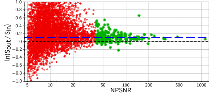
Fig. B.9. Comparison of FFP8's full catalogue of bright source flux densities with BeeP 's SREF. Shown in red are the source flux estimates with NPSNR < 40 and in green those with NPSNR > 40 . The horizontal long-dashed blue line is the \ln(S_{\text{out}}/S_{\text{in}}) median (0.104) of the green subset. The strong outlier is the result of a mock source blended with a real one.
