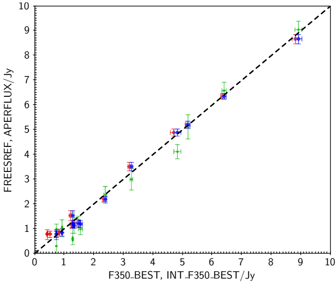
Fig. 28. Flux densities (FREESREF) of BeeP sources compared to those (F350_BEST) sources in the Herschel H-ATLAS GAMA15 field catalogue. The brightest H-ATLAS sources within 5' of the corresponding Planck source are shown in red. The beam-weighted sums of all sources within the corresponding Planck 857-GHz beam are shown in blue. Green symbols give a similar comparison between the Herschel beam-weighted flux-density sum and the PCCS2 APERFLUX flux density. The BeeP errors are not corrected here (see Sect. 6.2.4)
