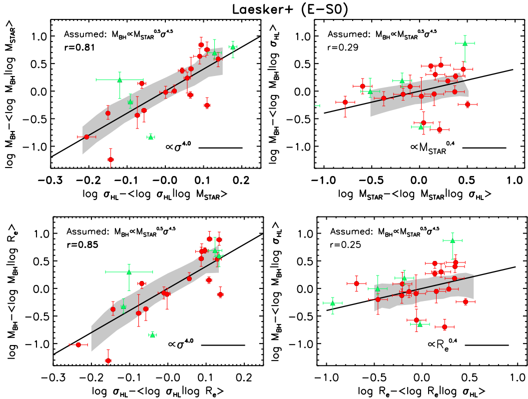
Figure A3. Same as Fig. 5 but using the E+S0 sample from Läscher et al. (2014). The data are consistent with velocity dispersion being the most fundamental property connecting black holes to galaxies.
