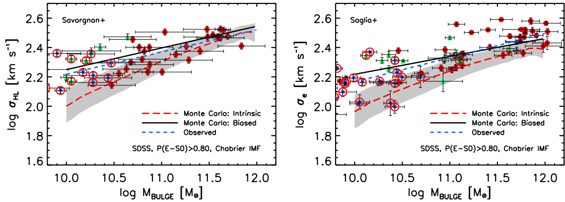
Figure 7. Left: same as top-right panel of Fig. 1 but with M_{\text{bulge}} rather than total M_{\text{star}} for the sample of Savorgnan et al. (2016). Right: same as left-hand panel but for the sample of Saglia et al. (2016), for which we have used \sigma_e as \sigma_{\text{HL}} is not available. We also include results of the Model I Monte Carlos when using only bulge stellar masses. Filled red circles, green triangles, and blue stars in both panels correspond, respectively, to ellipticals, S0, and the bulges of spirals. Open red circles mark the galaxies with bars. The predicted biased relations (black, solid lines) agree well with those observed (blue, dashed lines).
