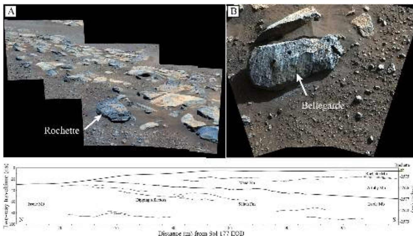
Figure 6. Mastcam-Z workspace mosaics and interpreted RIMFAX subsurface for Rochette: The Máaz formation outcrop target on top of Artuby Ridge and the first successful sample collected. (a) Shows Rochette that forms part of a NW—SE-trending band of similar boulders. (b) Rochette in which Bellegarde abrasion site and boreholes provide scale as in Figure 4.
