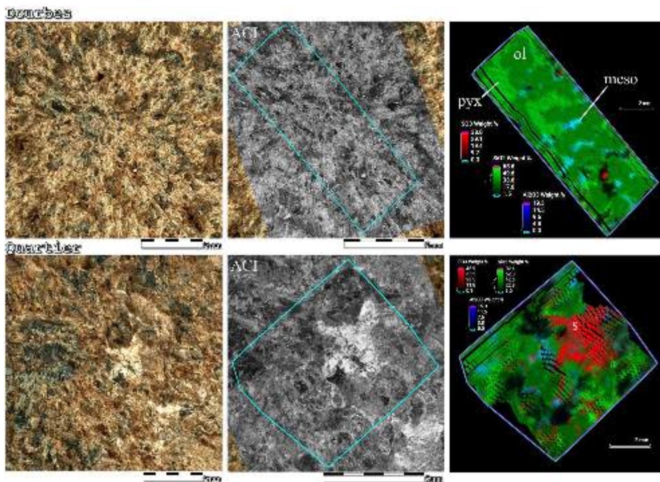
Figure 9. Close up observations of Séítah abrasion sites by WATSON (~4 cm standoff), Autofocus and Context imager, and PIXL: Compositional X-ray map of \text{SO}_3 (red), \text{SiO}_2 (green), and \text{Al}_2\text{O}_3 (blue) concentrations, generally correspond to primary olivine (ol) = dark green and pyroxene (pyx) = light green, compositionally evolved intercumulus mesostasis (meso) = blue and secondary sulfate (s) = red, respectively (see text and Figures S12–S16, Table S1 in Supporting Information S1 for additional information).
