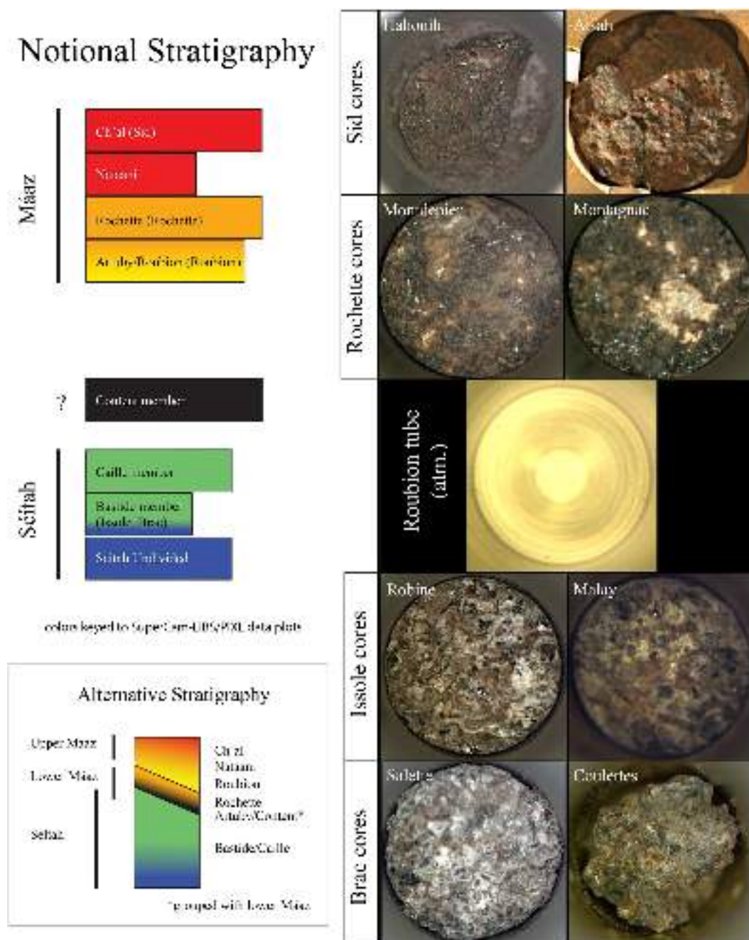
Figure 2. Samples from Jezero Crater floor collected by Perseverance: CacheCam images of rock sample cores from Séítah and Mááz units and tube of atmospheric gas prior to sealing. Core diameters are approximately 1.3 cm. Notional and alternative crater floor stratigraphic relationships of sampled units shown for reference (see Crumpler et al. (2023) and B. Horgan et al. (2022)).
