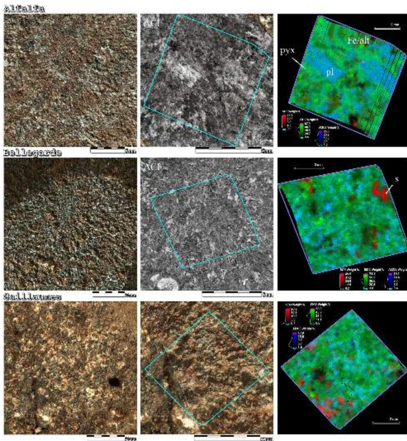
Figure 13. Close up observations of Máz abrasion sites by WATSON (~4 cm standoff), Autofocus and Context imager (ACI), and PIXL: Compositional X-ray map of \text{SO}_3 (red), \text{SiO}_2 (green), and \text{Al}_2\text{O}_3 (blue) concentrations, generally correspond to primary pyroxene (pyx) = light green, plagioclase (pl) = blue, and Fe-silicate/olivine (Fe/alt) = green and secondary sulfate (s) = red, respectively (see text and Figures S12–S16, Table S1 in Supporting Information S1 for additional information). Colorized ACI used to improve image clarity for Guillaume because of lighting conditions.
