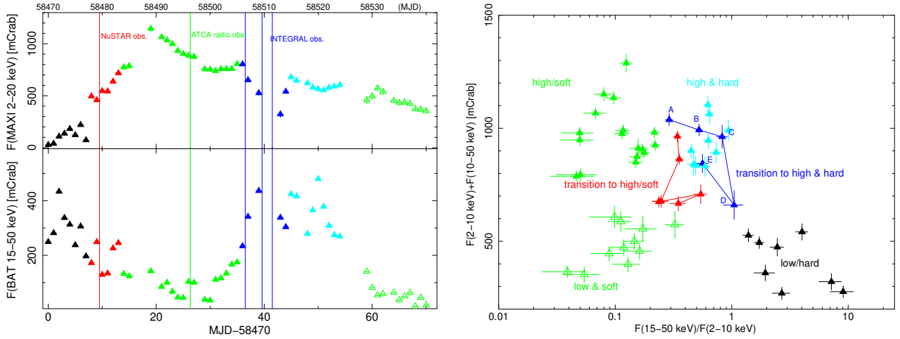
Figure 1. Left panel: the MAXI (upper) and Swift/BAT (lower) light curves of MAXI J1631–479, both with 1 day binning. Vertical lines indicate the time of the NuSTAR , ATCA and INTEGRAL observations. See text for details. Right panel: the hardness-intensity diagram with each point corresponding to 1 day: on the horizontal axis we show the ratio F_{(15-50 \text{ keV})}^{BAT}/F_{(2-10 \text{ keV})}^{MAXI} and in the vertical axis the total flux F_{(15-50 \text{ keV})}^{BAT} + F_{(2-10 \text{ keV})}^{MAXI} . Colored points indicate the different time intervals. Capitals letters indicate the time evolution of the hardness-intensity data during this transition, with A being the starting of the transition and E the end.
