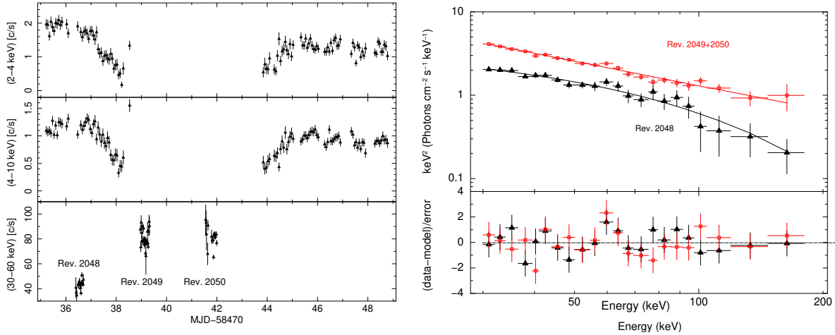
Figure 2. Left panel: Zoomed-in light curves during the INTEGRAL observation period, with the top (2-4 keV) and middle (4-10 keV) MAXI/GSC light curves (in 6h bins, data from http://maxi.riken.jp/top/slist.html ) compared with the bottom (30-60 keV) IBIS light curve (in 2000 s bins) over the three INTEGRAL revolutions. Right panel: INTEGRAL/IBIS unfolded spectra and residuals in sigma during revolution 2048 (in black) and during revolutions 2049 and 2050 (in red). Model is a cut-off power-law for the first data set and a simple power-law for the second one.
