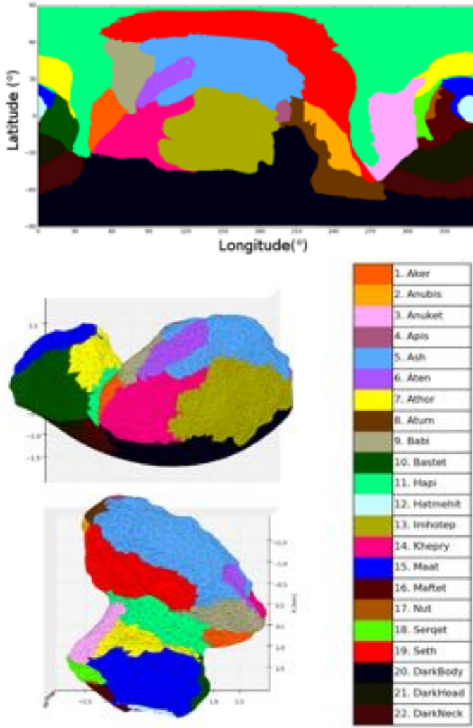
Fig. 7. Geomorphological regions of 67P in 2D and 3D visualization (after Thomas et al. 2015).
