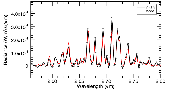
Fig. 4. VIRTIS-H spectrum of the 2.67 \mu\text{m} band of water. Average of 35 data cubes with most significant water and CO 2 detections (those with S/N > 10 ). The continuum has been subtracted. Superimposed we show a model spectrum of H 2 O band ( \nu_1 and \nu_3 ) for a rotational temperature T_{\text{rot}} = 102 \text{ K} (see text). The effective spectral resolution, derived from fitting, is R_{\text{eff}} = 800 .
