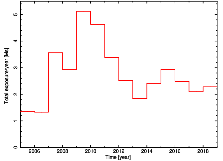
Fig. 1. Distribution of XRT exposure time in PC mode dedicated to known blazars over the 14 years of Swift mission operations covered in this work.
