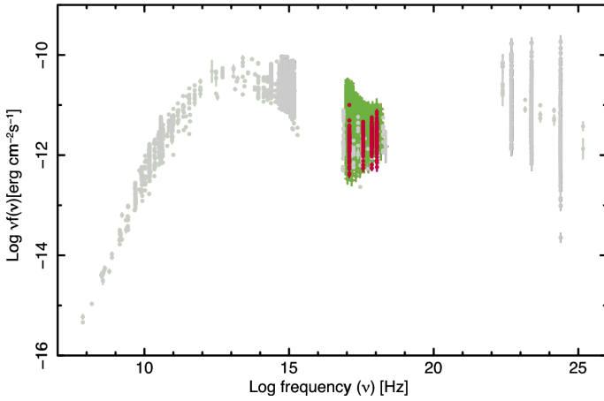
Fig. 7. Spectral energy distribution of the blazar OJ 287. The grey points are archival multi-frequency data. The red points are from this work (data in PC mode and count rate < 0.6 \text{ cts s}^{-1} ). The green points are XSPEC spectra from the first analysis of all the XRT data in PC and WT mode run on a small subsample of blazars (Giommi 2015).
