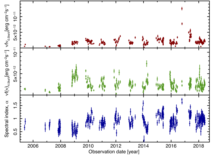
Fig. 8. \nu f(\nu) flux at 0.5, 4.5 keV and the power-law energy spectral index of the blazar OJ 287 are plotted against observation date. Many differences in the top and middle panels are clearly visible; in particular, the X-ray flares occur in different periods in the soft (0.5 keV) and hard (4.5 keV) parts of the X-ray spectrum.
