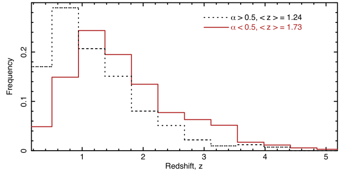
Fig. 11. Redshift distribution of FSRQs with different power-law spectral indices ( \alpha ). The black dotted histogram refers to objects with \alpha > 0.5 , while the red solid histogram is for sources with \alpha < 0.5 . FSRQs with flat spectral slopes tend to have higher redshifts.
