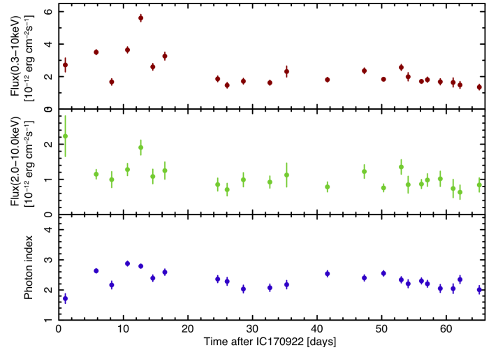
Fig. 9. 0.3–10.0 keV and 2–10 keV band flux in units of 10^{-12} \text{ erg cm}^{-2} \text{ s}^{-1} ( top and middle panel), and the power-law photon index of TXS0506+056 ( bottom panel) are plotted as a function of time. All uncertainties are given at 1\sigma .
