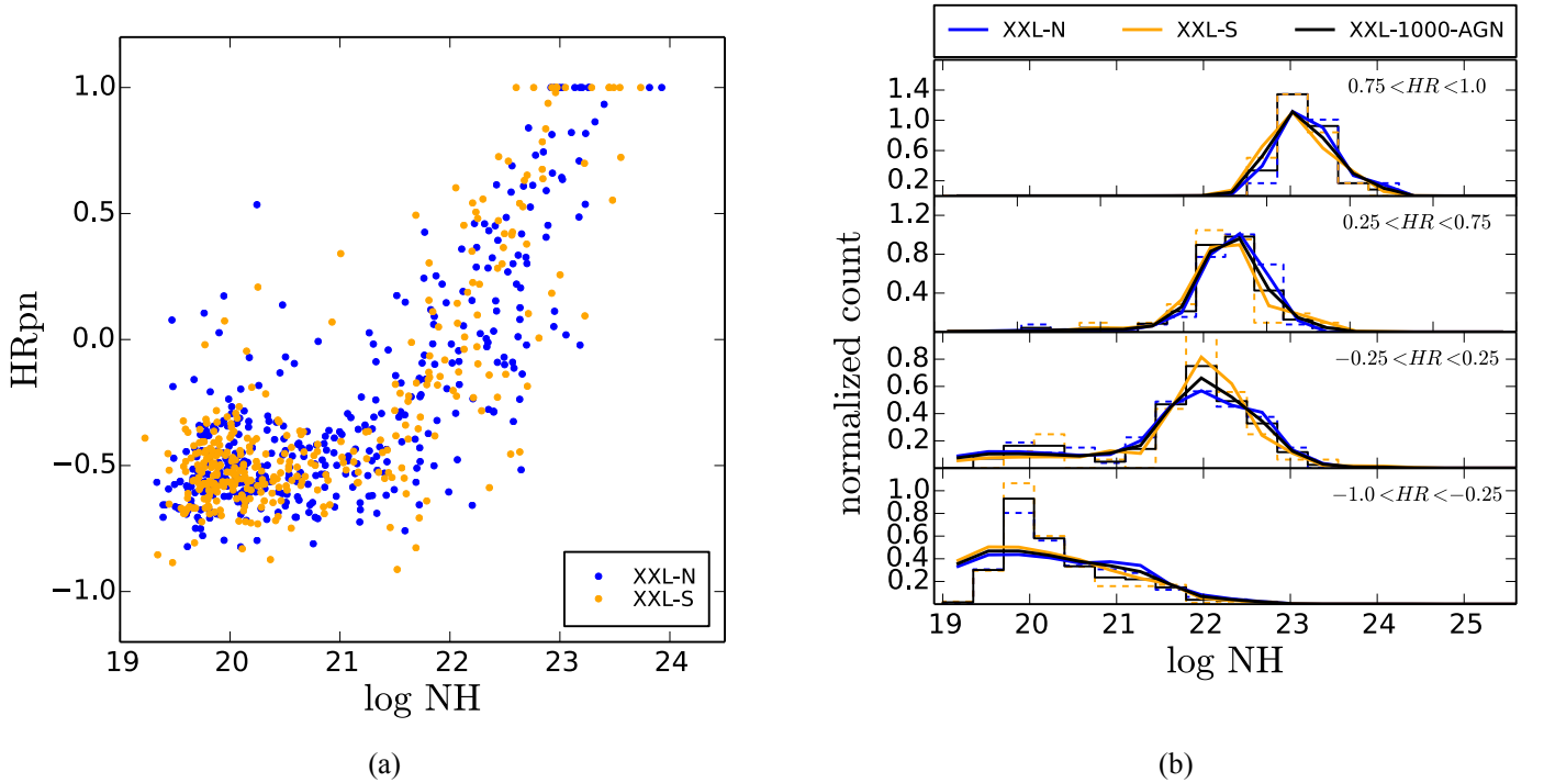
Fig. 6. a) Hardness ratio versus \log N_H for the XXL-N (blue points) and XXL-S (orange points); the hardness ratio is in good agreement with the estimated \log N_H from the X-ray spectra. b) \log N_H for four hardness ratio bins. The normalised dashed histograms represent the observed values in the XXL-N (blue) and XXL-S (orange) and the combined XXL-1000-AGN sample (solid black histogram). The solid lines show the combined \log N_H PDF of the sources in each bin (see Appendix B for the tabulated values of these curves).
