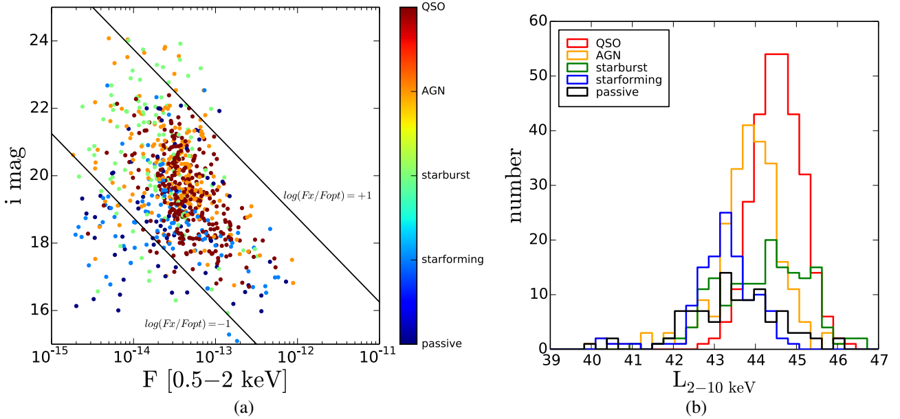
Fig. 3. a) F_X/F_{\text{opt}} diagram for the XXL-1000-AGN. The majority of the objects classified as quasi-stellar object (QSO)/AGN (red and orange dots) fall between the \log(F_X/F_{\text{opt}}) = \pm 1 lines, while passive objects (dark blue) and stars are gathered in the bottom left corner of the plot. b) X-ray luminosity per class. QSO classified objects have the highest 2–10 keV luminosity. The colour-coding indicates the photo- z class assigned by the Random Forest in both plots: QSO – red, AGN – orange, starburst – green, star forming – blue, passive – black.
