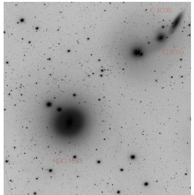
Figure 1. NGC 1533 sub-structure. VST deep image in the SDSS g-band of the IC 2038, IC 2039 (north west side) and NGC 1533 (south east side). The image size is 14' \times 14.7' . Astrosat-UVIT observations (see Table 1), cover the entire sub-structure.
