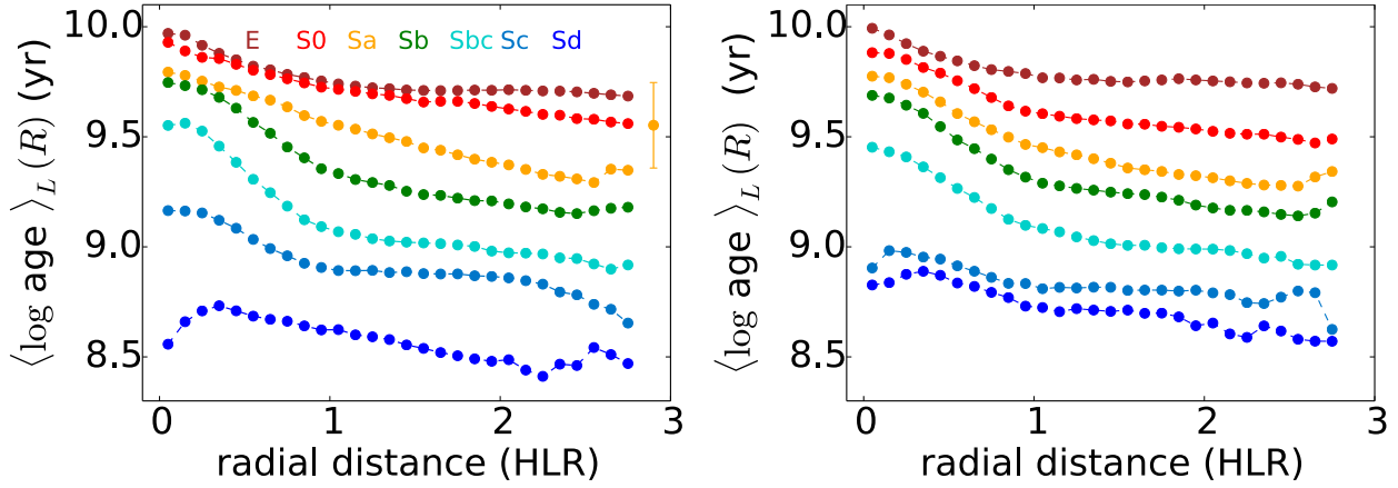
Fig. 9. Radial profiles of \langle \log \text{age} \rangle_L as a function of Hubble type ( left ) and in seven bins of galaxy stellar mass ( right ). These bins are \log M_*(M_\odot) = 9.1-9.6, 9.6-10.1, 10.1-10.6, 10.6-10.9, 10.9-11.2, 11.2-11.5, 11.5-11.8 . Symbols and colors are the same as in Fig. 6. These results are obtained with base GMe .
