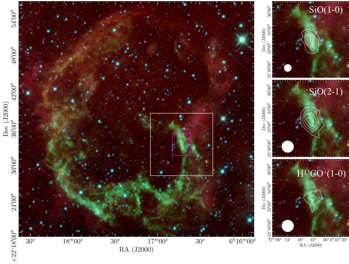
Figure 2. Left: Three-colour image (red = 22 \mu\text{m} ; green = 4.6 \mu\text{m} ; and blue = 3.4 \mu\text{m} ) of the SNR IC443 (WISE all-sky survey Wright et al. 2010). White and magenta rectangles indicate the extent of the ARO and Yebes maps, respectively. Right: Integrated intensity maps ( -22 ; 6 \text{km s}^{-1} ) of the SiO(1-0) (top; \sigma = 0.1 \text{ K km s}^{-1} ), SiO(2-1) (middle; \sigma = 0.2 \text{ K km s}^{-1} ), and \text{H}^{13}\text{CO}^+(1-0) (bottom; \sigma = 0.2 \text{ K km s}^{-1} ) are shown in white contours (from 3\sigma in steps of 3\sigma ). The ARO and Yebes beam sizes are shown as white circles in the bottom left of each panel.
