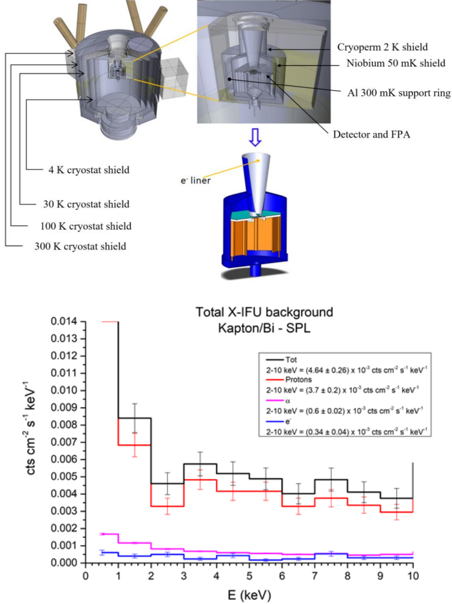
Fig. 1 Top and Center : the X-IFU mass model. On Top Left , the complete cryostat, on Top Right a zoom of the FPA region to highlight the detector hexagon in the center. In the Middle a sketch to show the electron liner shield. Bottom : expected residual background from the different particle species present in L2. The requirement is 0.005 cts/cm 2 /s/keV (error is due to statistics, the equivalent time of the simulations is several thousands of seconds). (Color figure online).
