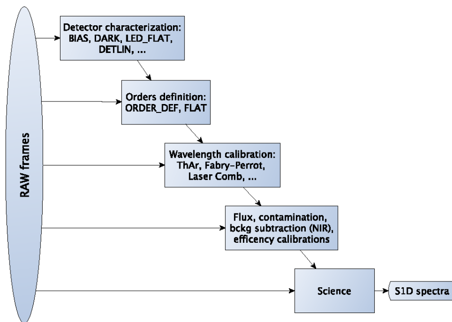
Figure 5. HIRES data reduction cascade.
