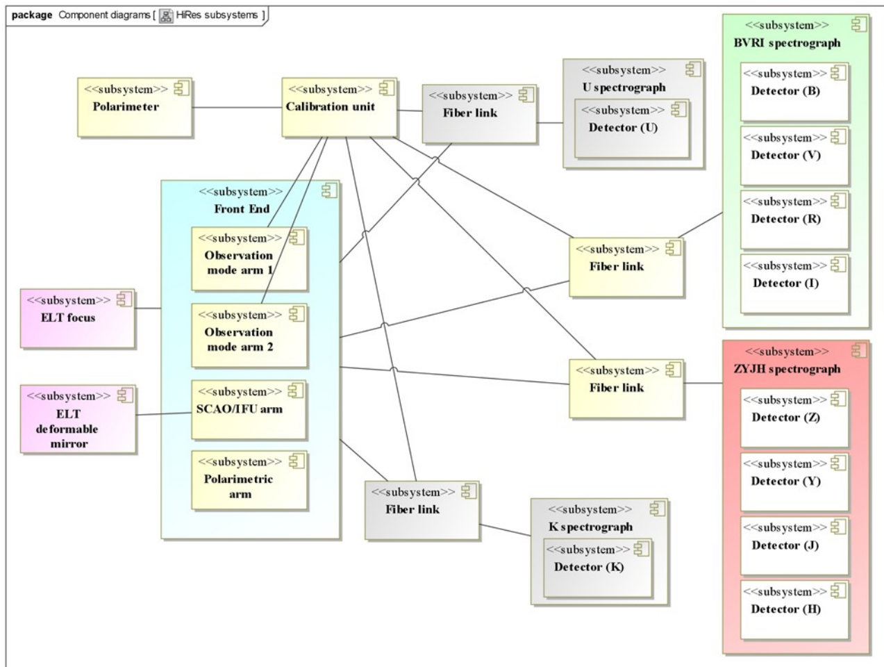
Figure 2. HIRES sub-systems. The grey boxes show the U and K spectrographs currently considered “ add-on ” due to cost cap imposed by ESO to all ELT second-generation instruments (see text for detailed description).
