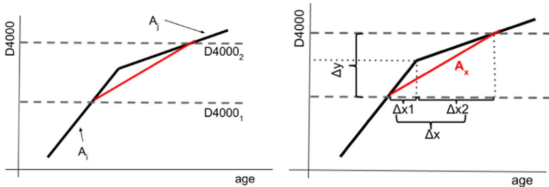
Figure A1. Estimating the correct piecewise linear slope across a knee. In the left panel, a schematic view of the D4000 -age relation is shown in black, where the dashed lines show the case of a measurement where the couple of D4000 values are located across a knee of the relation. In this case, it is incorrect to adopt the slopes A_i or A_j of the lower and upper part of the relation, but another slope should be estimated (shown in red). In the right panel, the various components of Equations (A1) and (A2) are shown, as well as the position of the knee (horizontal dashed line).
