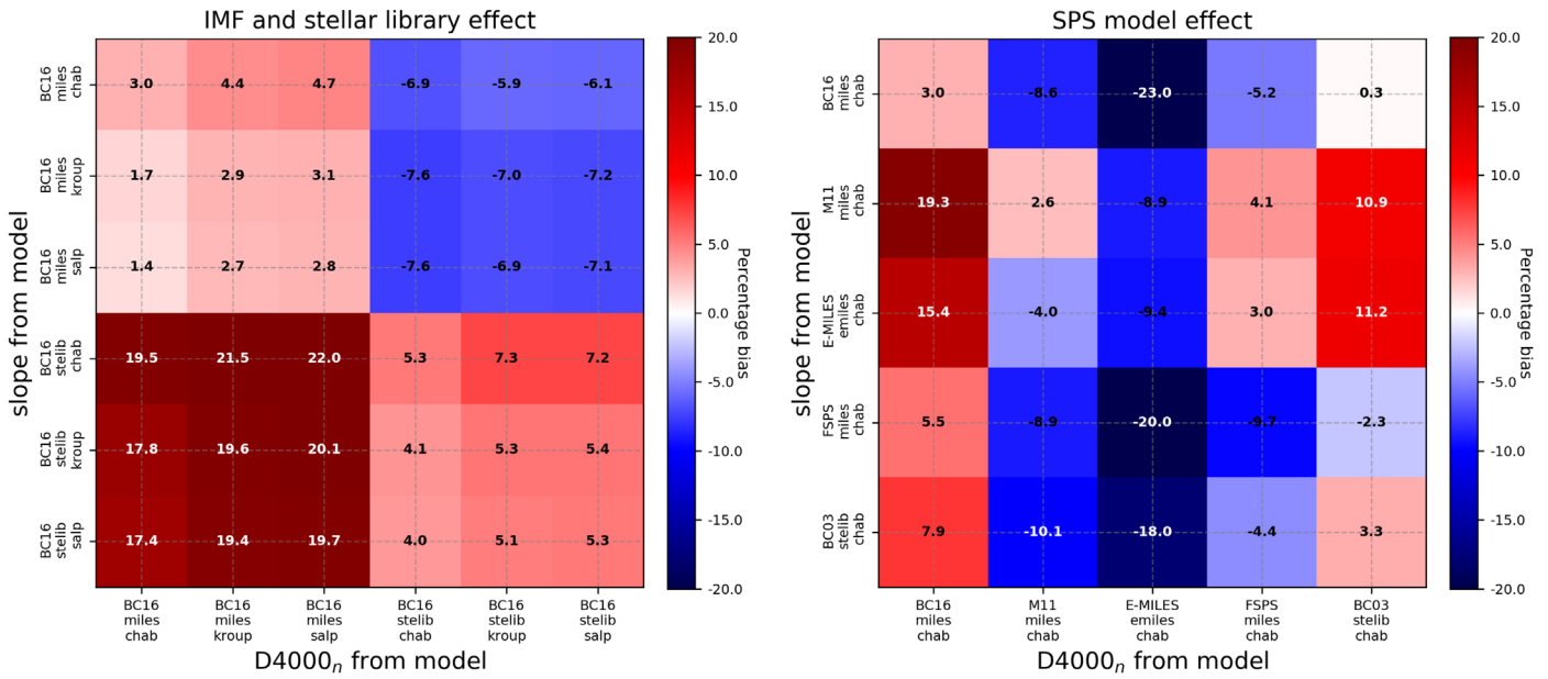
Figure B2. Same as Figure 4 but adopting the interpolated slope approach.
