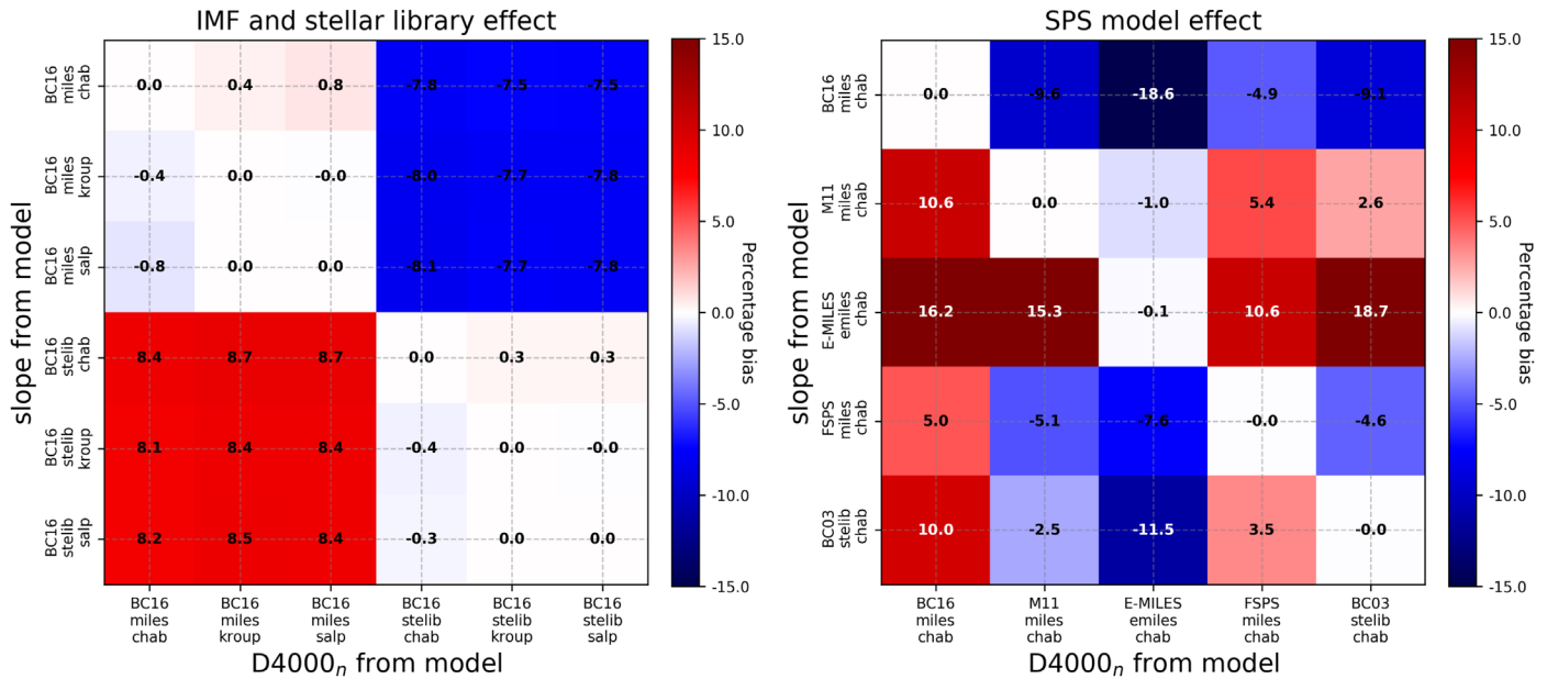
Figure 4. Matrix of the H(z) percentage difference as defined in Equation (7), where the x -axis label indicates from which model the D4000_n has been extracted, and the y -axis indicates from which model the slope A (see Equation (2)) has been extracted, considering a piecewise linear slope as discussed in the text. For illustrative purposes, we only show the matrix for 1.00 < z < 1.05 . In the left panel, we compare all models extracted from the BC16 SPS models, with different IMFs and stellar libraries as indicated in the caption, and in the right panels are shown models obtained with the same Chabrier IMF but from different codes. We also show the outdated BC03 models as a reference and not because they are being used in the current analysis, but they are an example of the level of model convergence and for reference for previous works.
