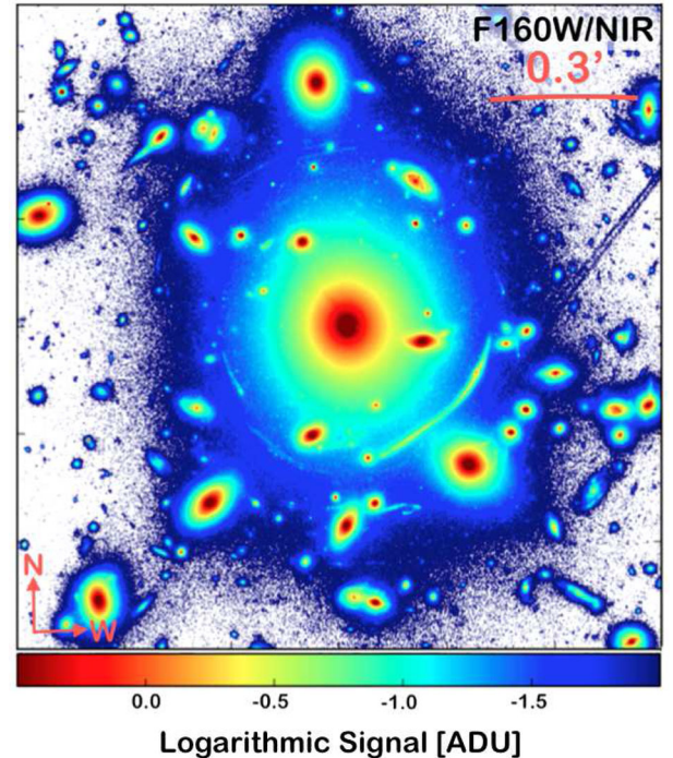
Figure 1. Example of the typical ICL+background signal contaminating the colours of the galaxies in the F160W/NIR image within the cluster Abell 383 ( z_s = 0.187 ).
