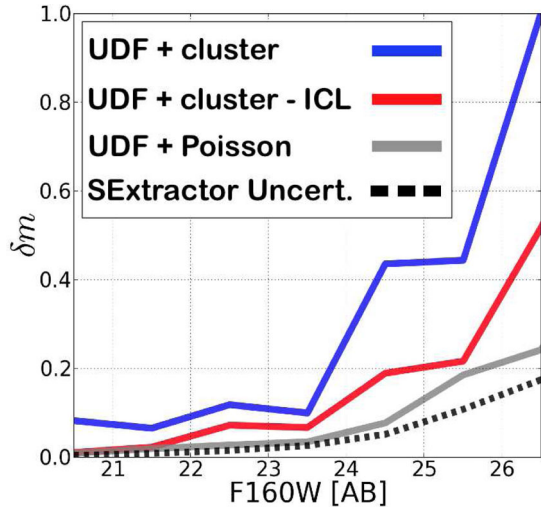
Figure 8. To study the reliability of SE EXTRACTOR deriving photometric uncertainties, galaxies from the UDF were injected in our images under different background conditions: instrumental background plus BCL (blue), instrumental background minus BCL (red) and pure Poisson background (grey). The observed variation of their original magnitudes ( \delta m ) as a function of a reference magnitude ( F160W ) showed that the uncertainties reported by SE EXTRACTOR were only accurately described for the Poisson case, but they were clearly underestimated for the CLASH images. As expected, the ICL subtraction (red) quantitatively improved the quality of our original photometry (blue).
