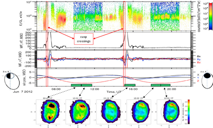
Figure 1. – June 7th 2012 time profiles. From top to bottom: FIPS proton spectrograms (the two cusp traversals are marked by red bars), MAG magnetic field (MF) magnitude, MAG MF components (MSO), s/c ephemeris components (MSO), the 1-hour-based Na dayside patterns observed by THEMIS. At the two sides of the ephemeris plot, s/c anti-clockwise orbital paths are shown. MESSENGER data are originated from the database server AMDA, http://amda.cdpp.eu . The color scale to the right relates to an intensity index that is normalized respect to the average Na intensity profile vs. TAA, as derived by [10].
