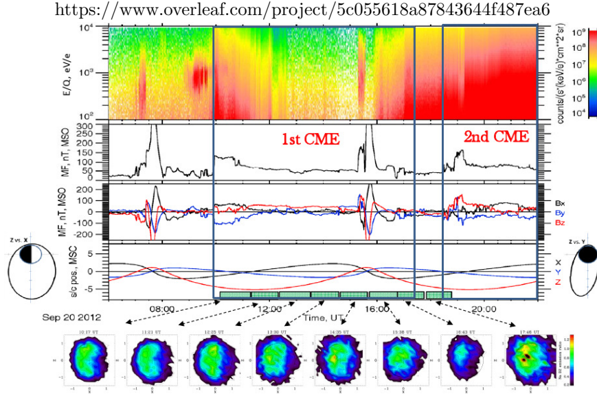
Figure 2. – September 20th 2012 time profiles (for description see Fig. 1). The arrival of two CMEs occurred at 09:53 and at 18:29.
