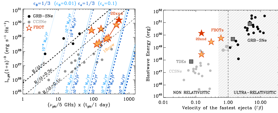
Figure 6. Left: radio phase space of stellar explosions, where L_{\nu, pk} is the spectral peak luminosity, \nu_{pk} is the spectral peak frequency, and t_{pk} is the peak time. Normal core-collapse stellar explosions (CCSNe, gray filled circles) typically show a shock velocity \sim 0.1c , while GRB-SNe (black filled circles) are characterized by significantly faster shocks. The new class of multiwavelength FBOTs (stars) currently comprises four elements and shows a variety of shock velocities that bridge the gap between normal SNe (e.g., AT 2018cow) and the ultrarelativistic jets of GRBs (e.g., CSS 161010, AT 2018lug, and AT 2020nxd). The dashed dark (dotted light) blue lines are lines of constant equivalent mass-loss rate for an assumed wind velocity v_w = 1000 \text{ km s}^{-1} for equipartition parameters \epsilon_B = \epsilon_e = 1/3 ( \epsilon_B = 0.01 , \epsilon_e = 0.1 ). Black dashed lines: lines of constant apparent velocity R/\Delta t under the assumption of equipartition. The factor (1+z)^{-3} accounts for the difference between the angular distance and the luminosity distance. Right: shock energy versus fastest ejecta velocity for a variety of transients, including TDEs, SNe, and FBOTs. FBOTs represent a new class of transients with energetic shocks that can be transrelativistic. Among FBOTs, AT 2020nxd shows the largest equipartition energy. The color coding is the same as in the left panel. The shaded region shows the parameter space of engine-driven explosions. References: Margutti et al. (2019); Ho et al. (2019b); Coppejans et al. (2020).
