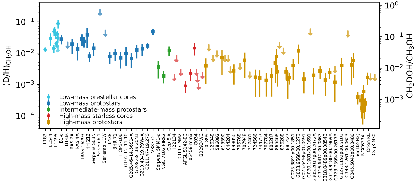
Fig. 3. (D/H)_{CH_3OH} ratio (squares) derived from the N_{CH_2DOH}/N_{CH_3OH} for low-mass, intermediate-mass, and high-mass protostellar systems including data from both this study and the literature (see Appendix C for references). Only D/H ratios derived from interferometric observations are included to minimize effects of beam dilution and to exclude any contribution from larger scales. Also data for low-mass prestellar cores and high-mass starless cores (circles) from the literature (including observations with single dish telescopes) are included. Upper limits are presented as arrows.
