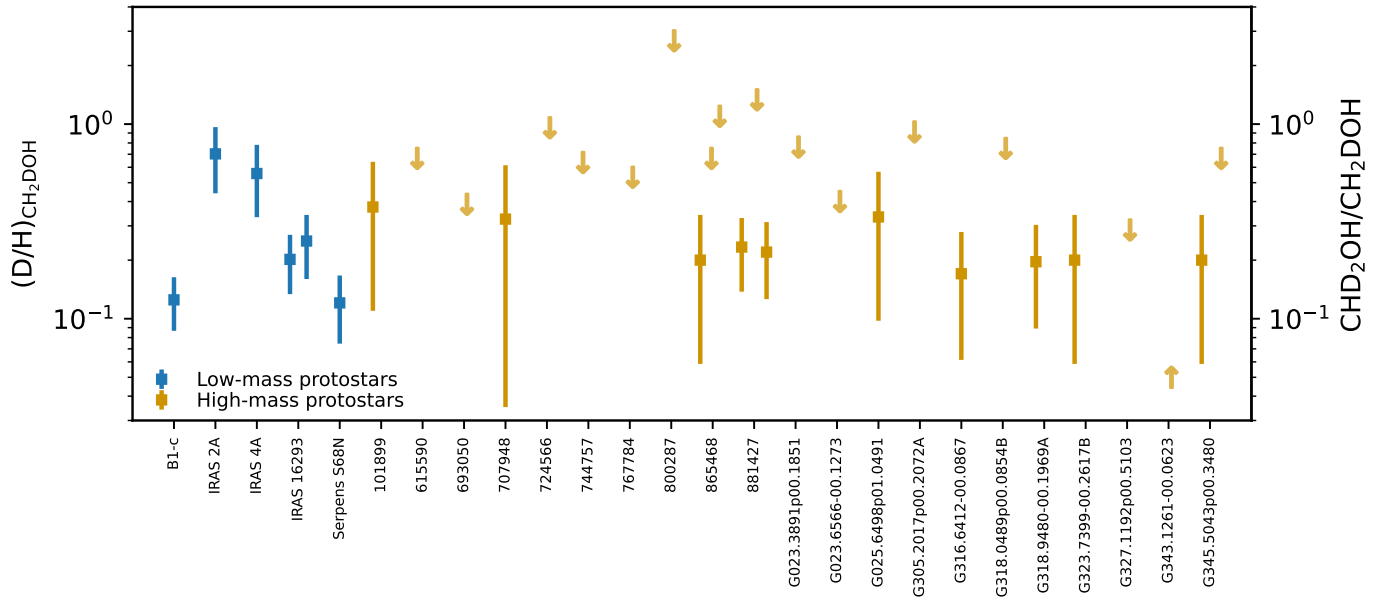
Fig. 4. (D/H)_{CH_2DOH} ratio derived from the N_{CHD_2OH}/N_{CH_2DOH} for low-mass and high-mass protostellar systems including data from both this study and the literature (see Appendix C for references). Upper and lower limits are presented as arrows. Only D/H ratios derived from interferometric observations are included to minimize effects of beam dilution and to exclude any contribution from larger scales. The (D/H)_{CH_2DOH} of IRAS 2A and IRAS 4A were derived using older spectroscopic data (Taquet et al. 2019).
