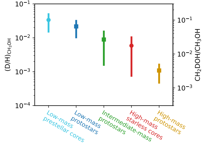
Fig. 5. Average (D/H)_{CH_3OH} ratio derived from N_{CH_2DOH}/N_{CH_3OH} for low-mass, intermediate-mass, and high-mass protostellar systems and low-mass prestellar cores and high-mass starless cores. The prestellar phases are indicated with circles and the protostellar phases with squares.
