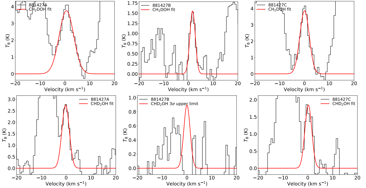
Fig. 2. Spectral line fits of CH 2 DOH 17_{1,16} e_0 - 17_{0,17} e_0 ( E_{\text{up}} = 336 K, top row ) and CHD 2 OH 7_{0,1} e_1 - 6_{1,1} e_1 ( E_{\text{up}} = 74 K, bottom row ) for 881427A ( left ), 881427B ( middle ), and 881427C ( right ). The data corrected for the V_{\text{lsr}} are shown in black and the best fit for T_{\text{ex}} = 150 K is shown in red.
