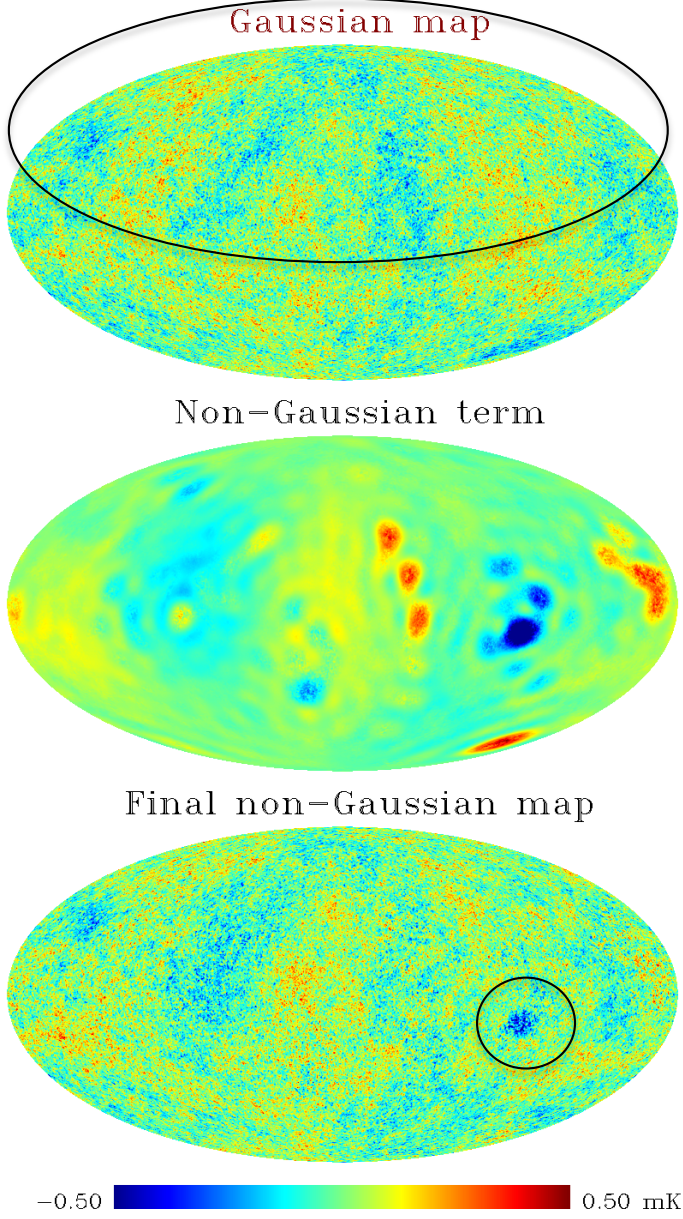
Fig. 4. Cold spot with the hot ring from the simulation shown in Fig. 3
