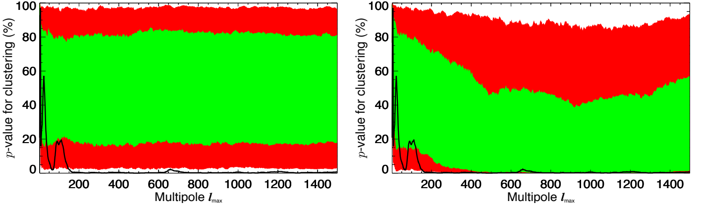
Fig. 7. p -values for alignment of the spatial power distribution dipoles up to a given multipole. This is the equivalent plot to figure 36 in Planck Collaboration XVI (2016). The green and red bands indicate the 1\sigma and 2\sigma spread of p -values measured in 1000 Gaussian simulations (left panel) and 1000 non-Gaussian model simulations (right panel). The black line corresponds to the p -values for Planck data taken from figure 36 in Planck Collaboration XVI (2016). These p -values show the percentage of Gaussian simulations with a larger alignment of the spatial power distribution up to the given multipole (calibrated with 1000 Gaussian simulations).
