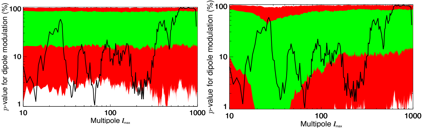
Fig. 6. p -values for dipolar modulation, to be compared with figure 30 in Planck Collaboration XVI (2016). Green and red bands show the 1\sigma and 2\sigma spread of p -values measured in 1000 Gaussian simulations (left plot) and 1000 non-Gaussian model simulations (right plot). In both plots, the black line shows the p -values for Planck data taken from figure 30 in Planck Collaboration XVI (2016). These p -values show the percentage of Gaussian simulations having larger dipolar modulation up to the given multipole than the Planck data (calibrated with 1000 Gaussian simulations).
