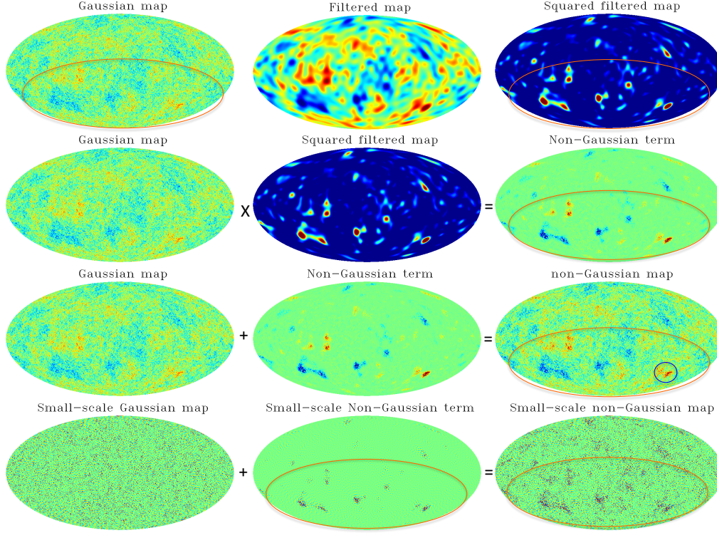
Fig. 1. First row: Gaussian CMB realisation (left), the filtered version (middle), and the square of the filtered map (right). The orange ellipse denotes the random dipole direction observed on large angular scales. For the squared map, dark blue corresponds to zero temperature, while for all other maps dark red and dark blue correspond to the largest negative and positive fluctuations in the map. Second row: Product of the Gaussian map (left) and the squared filtered map (middle) generates the non-Gaussian contribution (right) that enhances the dipole in the power distribution. Third row: Combination of the original Gaussian map (left) and the non-Gaussian term (middle) scaled by the factor \beta_{\text{dimensionless}} = 1.77 \times 10^8 yielding a non-Gaussian map (right) with enhanced dipole modulation and a hot spot with excess kurtosis shown in the blue circle. Last row: As in the third row, but for scales \ell = 100 - 200 only. The value of \beta is exaggerated here in order to make the effect visible by eye.
