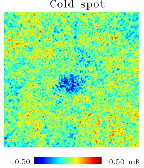
Fig. 4. Cold spot with the hot ring from the simulation shown in Fig. 3
