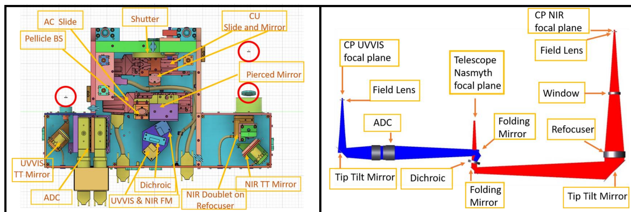
Figure 1. Mechanical (left) and optical (right) sketches of the SOXS Common Path. The optical components (UUVIS field lens, NIR window and NIR field lens) in the red circles are formally a part of the CP, but their mechanical mount should fit the mechanical benches of the spectrographs.
