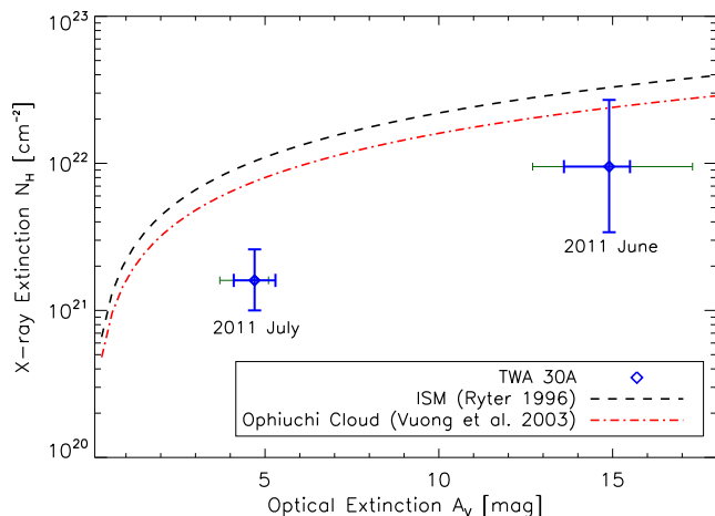
Figure 7. The relationship between gas ( N_{\text{H}} ) and dust ( A_{\text{V}} ) extinction in TWA 30A for two epochs of contemporaneous observations compared to the ISM (black dashed line; Ryter 1996) and the \rho Ophiuchi molecular cloud (red dash-dotted line; Vuong et al. 2003), all of which assume that an R_{\text{V}} = 3.1 . For each observation, the uncertainty in the determinations of A_{\text{V}} corresponding to a plausible range of R_{\text{V}} for dust in the TWA 30A disc (i.e. R_{\text{V}} = 2.75 to 5.3 ; see Sections 3.1, 4.2) is shown as a green error bar.
