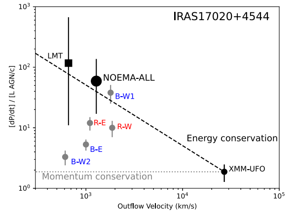
Figure 3. This plot shows the relative force of the molecular and X-ray phases of the wind (expressed as the ratio of their momentum rates divided by the AGN radiation momentum rate) plotted against their respective outflow velocities for IRAS17: the grey circles mark the five NOEMA wind components reported in Table 1. The red and blue labels for these points refer, respectively, to the receding and approaching velocities of the CO gas. The black circles mark the X-ray UFO from XMM-Newton (Longinotti et al. 2015) and the total molecular outflow obtained by combining the five NOEMA components. The black square marks the former detection of the molecular outflow observed with the LMT (Longinotti et al. 2018). The black dashed line marks the prediction for the energy conserving outflow in the B-W1 component i.e. \dot{P}_{[\text{CO}]} / \dot{P}_{[\text{X}]} = v_{\text{out,X}} / v_{\text{out,CO}} . The grey dotted line marks the prediction for momentum-conserving outflows.
