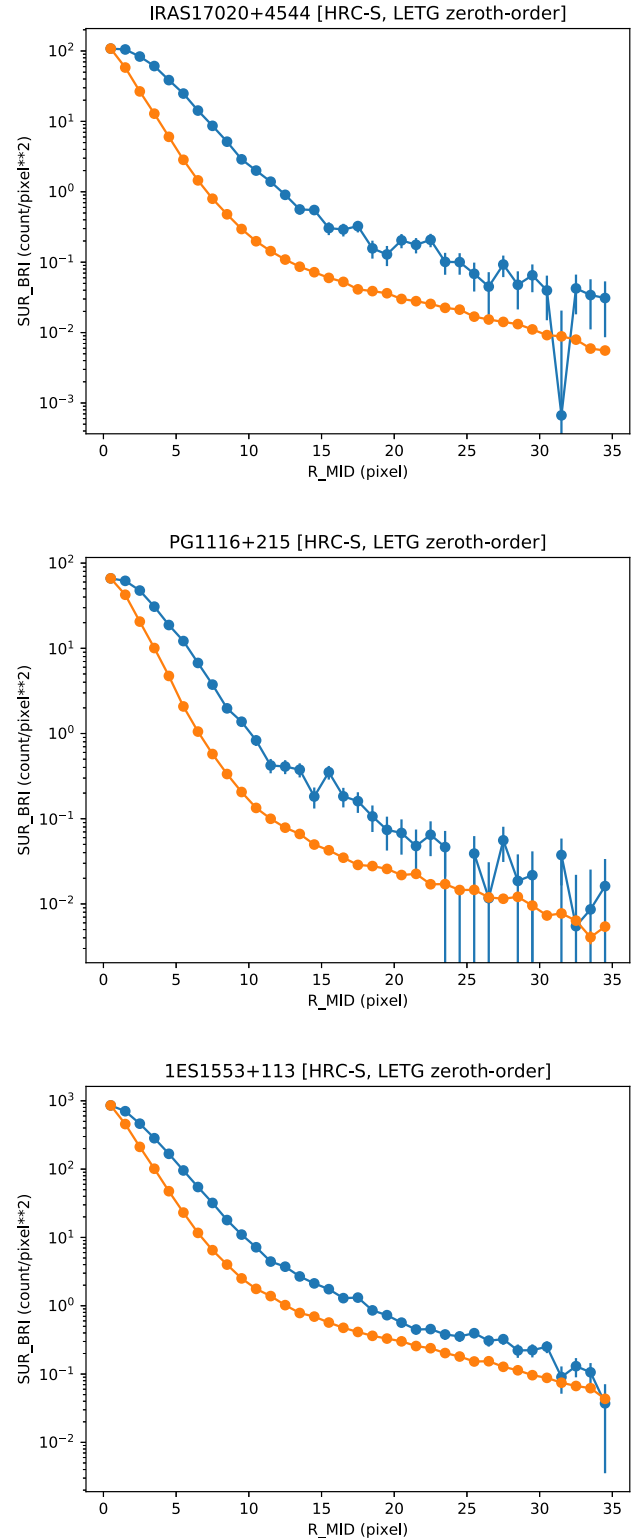
Figure A1. Comparison of the radial brightness profile of the source (blue) and PSF (orange) obtained by ray-tracing with ChaRT for IRAS17 and for the other two comparison sources: PG1116+215 and 1ES1553+113.
