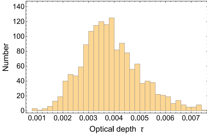
Fig. 13. Histogram of the optical depth \tau derived using Eq. (29) for 1526 X-ray cluster positions.
