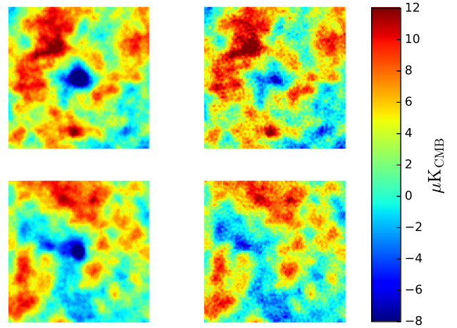
Fig. 1. Top left: stack of the NILC CMB map in the directions of Planck SZ (PSZ) galaxy clusters. Top right: stack of the 2D-ILC CMB map in the direction of PSZ galaxy clusters. This sample provides a very stringent test of the tSZ leakage, since the PSZ positions are the known places on the sky with detectable SZ signal. The stacked NILC CMB map clearly shows an excess in the centre, which is due to residual contamination from the tSZ effect, while the 2D-ILC CMB map has a signature in the centre that is consistent with the strength of other features in the stacked image. Bottom left: stack of the NILC CMB map in the directions of MCXC clusters. Bottom right: stack of the 2D-ILC CMB map in the direction of 1526 MCXC clusters (see Sect. 2.2 for the detail of the catalogue). For a different set of sky positions, the results are broadly consistent with those for the PSZ clusters. All these maps are 3^\circ \times 3^\circ in size, and use the same colour scale.
