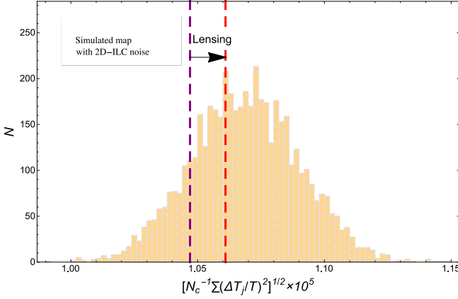
Fig. 12. Histogram of the [N_c^{-1} \sum_j (\Delta T_j / T)^2]^{1/2} values of 5000 random catalogues (each having N_c = 1526 ) on simulated lensed skies with added 2D-ILC noise. The mean and rms for the 5000 mock catalogues are 1.07 \times 10^{-5} and 2.13 \times 10^{-7} , respectively. The vertical dashed lines indicate the values at the MCXC cluster positions before and after the cluster-lensing effect is added; the values are 1.047 \times 10^{-5} before (purple line) and 1.061 \times 10^{-5} after (red line).
