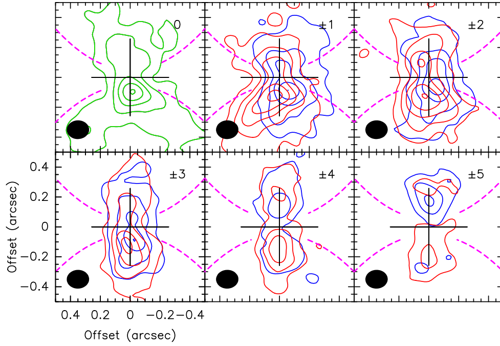
Fig. A.1. Channel maps of continuum-subtracted \text{SO}_2 8(2,6) - 7(1,7) emission within \pm 0.5'' of the central source of HH212. The velocity offset from the systemic velocity ( V_{\text{sys}} = 1.7 \text{ km s}^{-1} ) is indicated (in \text{km s}^{-1} ) in the upper right corner with blue and red contours denoting blueshifted and redshifted emission. The channel width is 1 \text{ km s}^{-1} . First contour and steps corresponds to 4\sigma and 6\sigma ( \sigma = 1 \text{ mJy/beam} ), respectively. The \text{C}^{34}\text{S} cavity boundary from Fig. 1 is drawn in magenta dashed lines.
