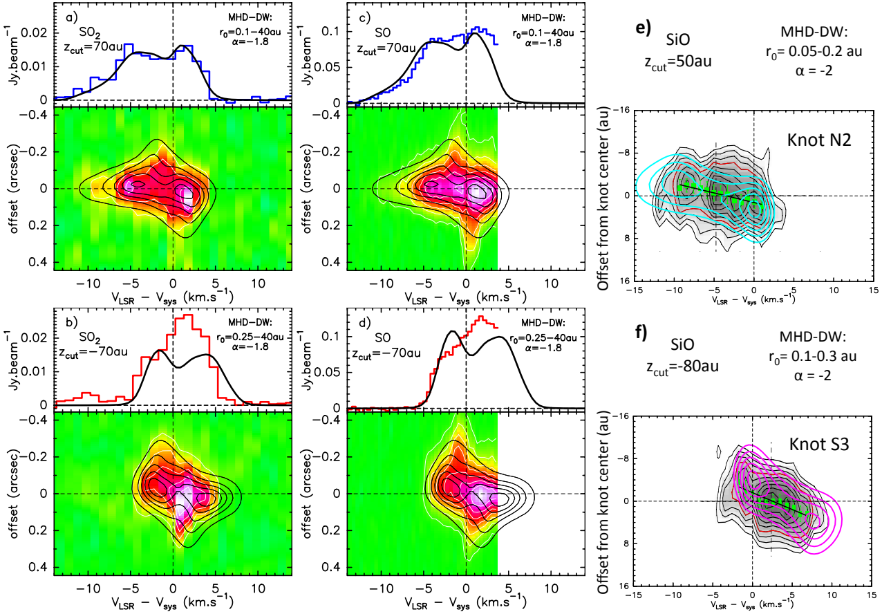
Fig. 2. a-d: Observed on-axis line profiles (histograms) and transverse PV diagrams (color map and white contours) of SO 2 (left) and SO (middle) at \pm 70 au across the northern blue jet (top) and the southern red jet (bottom). The red wing of SO falls outside our spectral set-up. A DW model fit, with \lambda = 5.5 and \mathcal{W} = 30 (see text), is overplotted in black for parameters denoted in each panel. e-f: PV diagrams observed by Lee et al. (2017a) across the SiO knots N2 and S3 (grayscale and black/red contours). Their measured centroids are shown as green squares and fitted rotation gradient as a black line. The DW model is overplotted in cyan (top) or magenta (bottom) with parameters denoted above each panel.
