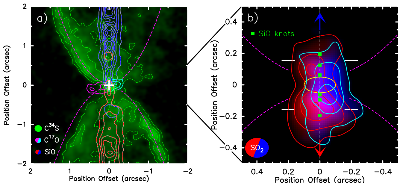
Fig. 1. a: HH212 inner region viewed by ALMA Cycle 4. The SiO jet at |V_{LSR} - V_{sys}| = 5\text{--}10\text{ km s}^{-1} (blue and red contours), \text{C}^{17}\text{O} rotating envelope at |V_{LSR} - V_{sys}| = 1.5\text{ km s}^{-1} (pink and turquoise), and cavity walls in \text{C}^{34}\text{S} at |V_{LSR} - V_{sys}| \leq 0.6\text{ km s}^{-1} (green, with parabolic fits in dashed magenta) are shown. First contour and step are 6\sigma and 18\sigma for SiO, 6\sigma and 6\sigma for \text{C}^{17}\text{O} , 4\sigma and 4\sigma for \text{C}^{34}\text{S} , where \sigma is the rms noise level. The source is shown as a white cross and beam sizes are in the bottom left corner. b: Zoom-in on blue and red \text{SO}_2 at \pm 2\text{ km s}^{-1} shows a slow outflow rotating in the same sense as the \text{C}^{17}\text{O} disk. First contour and step are 7\sigma . White segments show the positions of PV cuts in Fig. 2. Green squares show inner SiO knots imaged by Lee et al. (2017a); the yellow ellipse marks the centrifugal barrier radius at r \sim 45\text{ au} and the height of the COM-rich disk atmosphere at z \pm 20\text{ au} (Lee et al. 2017c). Images are rotated such that the vertical axis corresponds to the jet axis at P.A. = 22^\circ .
