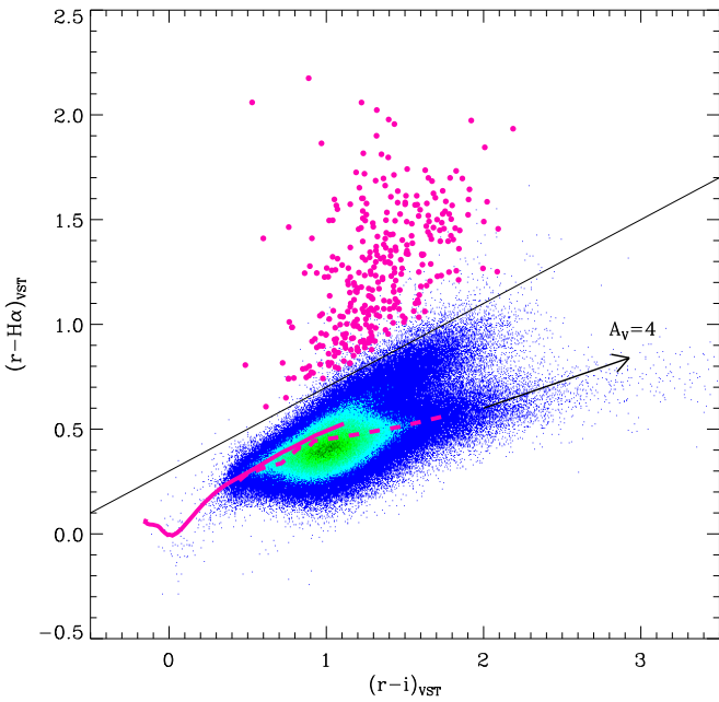
Fig. 2. VST r-H\alpha vs. r-i diagram plotted as a two-dimensional stellar-density histogram using a binning of 0.005 \times 0.005 and an eight-level color-coded scale such that high source densities (130 per bin) are dark green and the lowest densities (one per bin) are violet. The magenta solid and dashed lines are the synthetic unreddened main sequence and giant loci, respectively, given by Drew et al. (2014) , and the black solid line is the limit adopted to select objects with H\alpha excesses, drawn as magenta circles.
