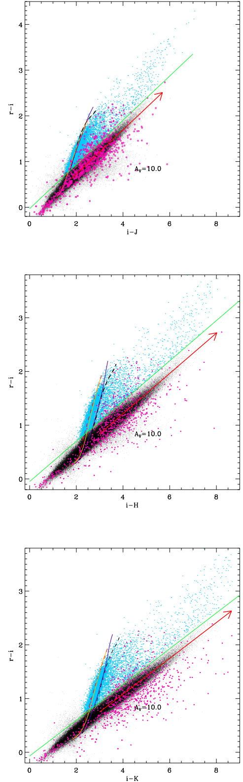
Fig. 13. r-i vs. i-J , i-H , and i-K diagrams plotted as a two-dimensional stellar density histogram on a gray scale, compared with the MS locus (dashed red line), the 10 Myr and 0.5 Myr isochrones (orange and purple lines), and the giant locus (black line) predicted by PISA models. YSOs selected with classical methods and objects selected as M-type stars are indicated with magenta and cyan symbols, respectively. The reddening vectors and the limits used for the selection of M-type stars are indicated as red arrows and green lines, respectively.
