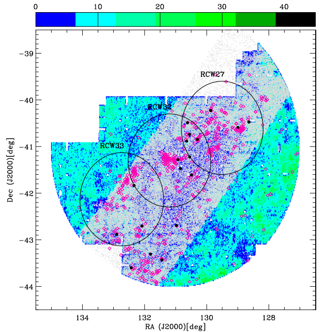
Fig. 9. Spatial distribution as in Fig. 3, where all the Spitzer /IRAC sources are overplotted with gray symbols. YOSs with IR excesses are indicated as in Fig. 5. The three circular boundaries delimit the regions of the three clusters.
