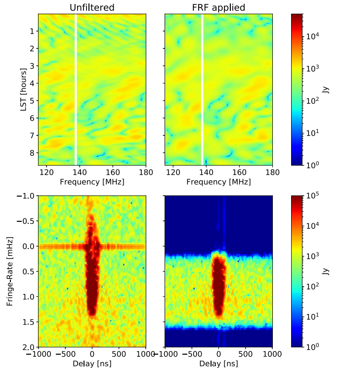
Figure 7. Top: LST and frequency waterfalls of representative baselines taken from the even LST-binned set before (left) and after (right) application of the top-hat FRF. The baseline illustrated is the antenna pairs (1, 4). The application of the fringe-rate filter removes very fast fringe modes but preserves the structure of sky-like modes. Bottom: the same baseline before (left) and after (right) the application of the FRF plotted in fringe rate and delay space. The Fourier representation of the data illustrates the common mode at fringe rate = 0 mHz suppressed by the filter.
