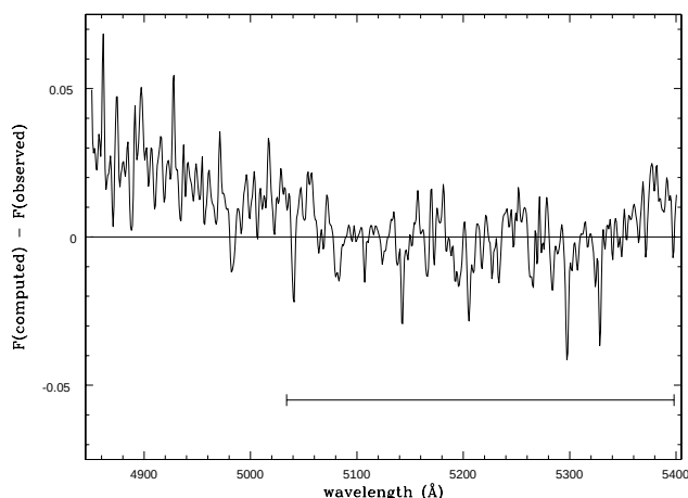
FIG. 1.—Difference between computed and observed absolute flux for the solar spectrum, degraded and rebinned according to the characteristics of the program stars spectra. The 5034–5398 \text{\AA} interval is indicated.
