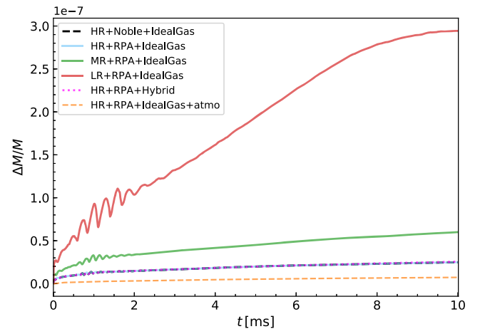
FIG. 3. Relative change in total baryonic mass for the different tests with Noble and RePrimAnd schemes.
